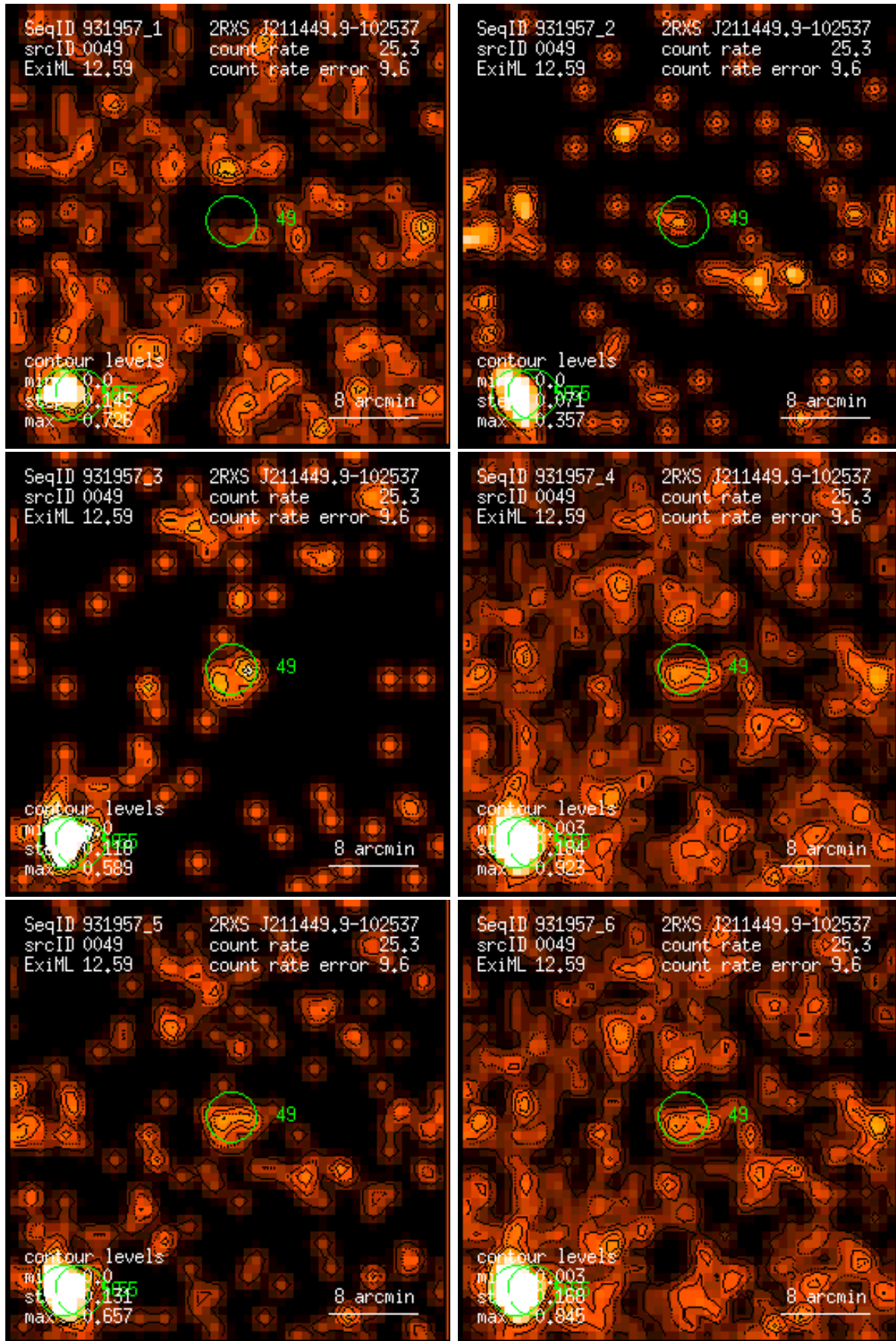
Figure 49: RASS 931957: detection 0049: band rate images, Gaussian filter: (1) PSPC channels 11 – 41, (2) 52 – 90, (3) 91 – 201, (4) 11 – 235, (5) 52 – 201, (6) 11 – 201. Broad band rates in counts/ks. Band rate contour levels in counts/ks/arcmin 2 .
