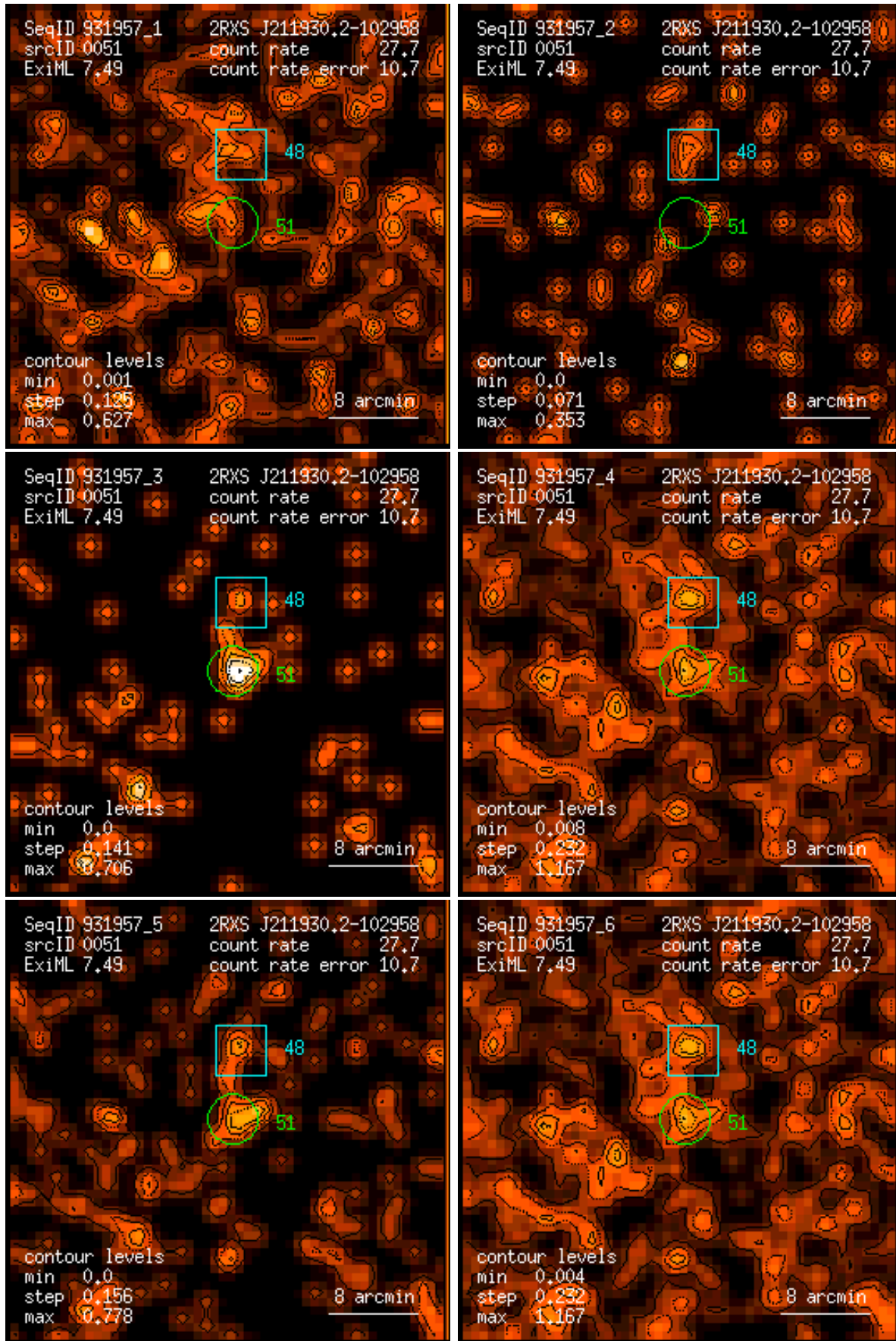
Figure 51: RASS 931957: detection 0051: band rate images, Gaussian filter: (1) PSPC channels 11 – 41, (2) 52 – 90, (3) 91 – 201, (4) 11 – 235, (5) 52 – 201, (6) 11 – 201. Broad band rates in counts/ks. Band rate contour levels in counts/ks/arcmin 2 .
