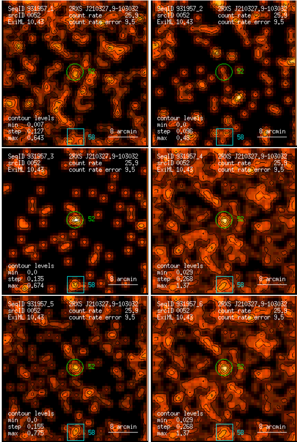
Figure 52: RASS 931957: detection 0052: band rate images, Gaussian filter: (1) PSPC channels 11 – 41, (2) 52 – 90, (3) 91 – 201, (4) 11 – 235, (5) 52 – 201, (6) 11 – 201. Broad band rates in counts/ks. Band rate contour levels in counts/ks/arcmin 2 .
