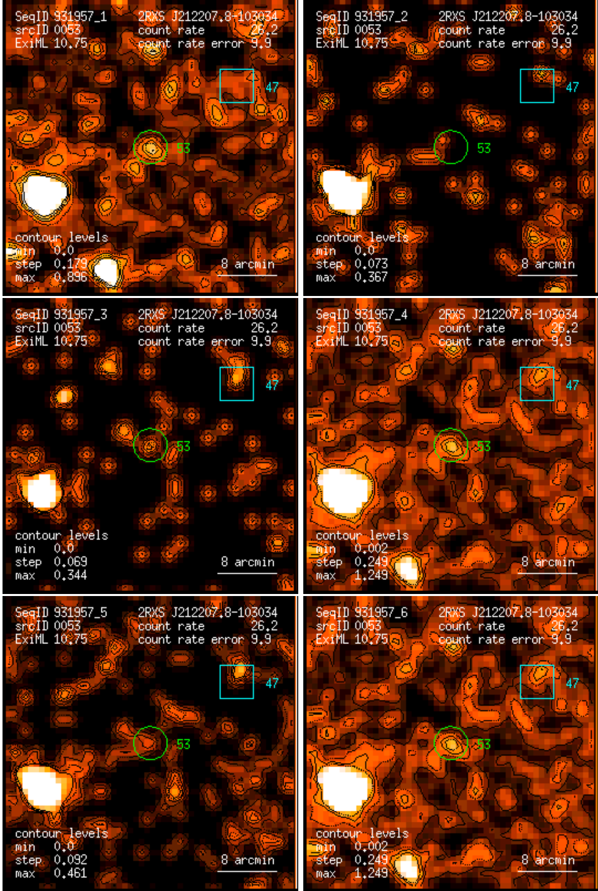
Figure 53: RASS 931957: detection 0053: band rate images, Gaussian filter: (1) PSPC channels 11 – 41, (2) 52 – 90, (3) 91 – 201, (4) 11 – 235, (5) 52 – 201, (6) 11 – 201. Broad band rates in counts/ks. Band rate contour levels in counts/ks/arcmin 2 .
