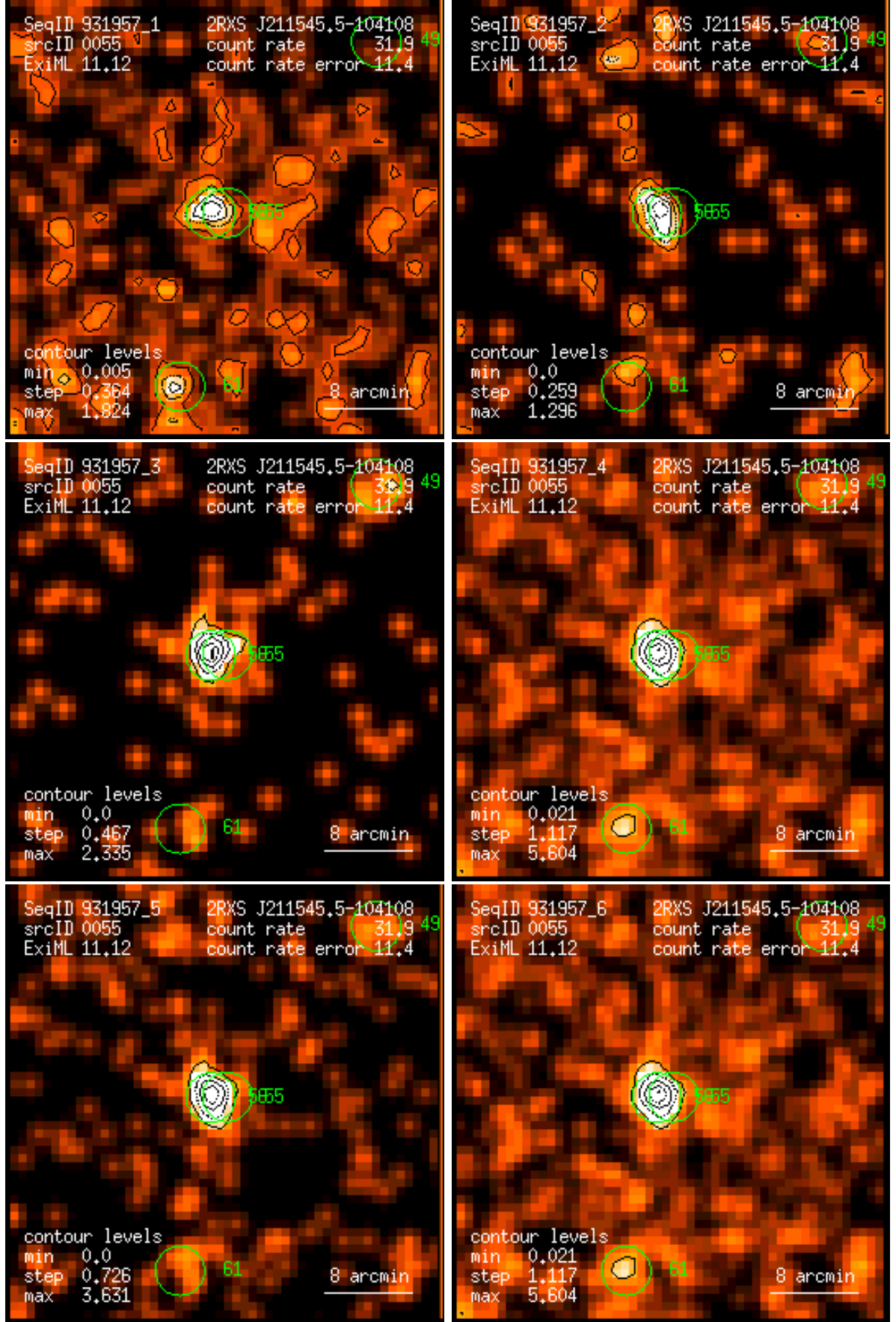
Figure 55: RASS 931957: detection 0055: band rate images, Gaussian filter: (1) PSPC channels 11 – 41, (2) 52 – 90, (3) 91 – 201, (4) 11 – 235, (5) 52 – 201, (6) 11 – 201. Broad band rates in counts/ks. Band rate contour levels in counts/ks/arcmin 2 .
