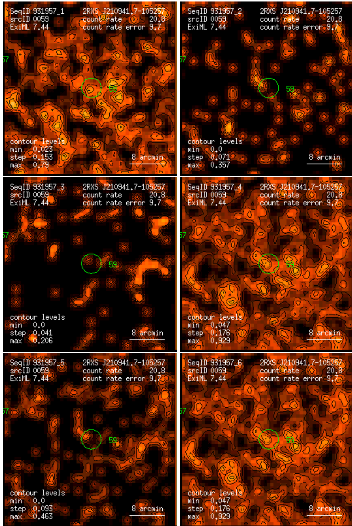
Figure 59: RASS 931957: detection 0059: band rate images, Gaussian filter: (1) PSPC channels 11 – 41, (2) 52 – 90, (3) 91 – 201, (4) 11 – 235, (5) 52 – 201, (6) 11 – 201. Broad band rates in counts/ks. Band rate contour levels in counts/ks/arcmin 2 .
