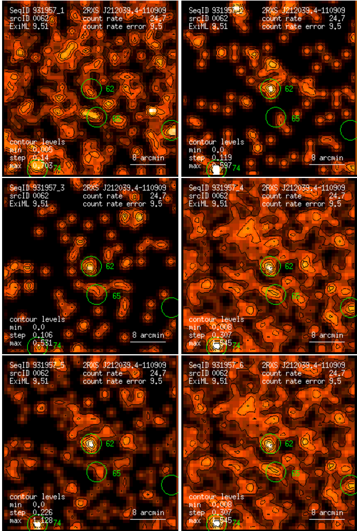
Figure 62: RASS 931957: detection 0062: band rate images, Gaussian filter: (1) PSPC channels 11 – 41, (2) 52 – 90, (3) 91 – 201, (4) 11 – 235, (5) 52 – 201, (6) 11 – 201. Broad band rates in counts/ks. Band rate contour levels in counts/ks/arcmin 2 .
