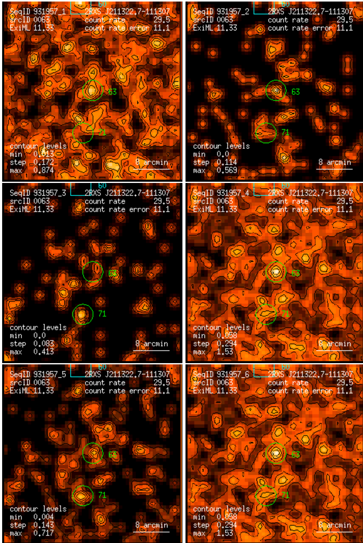
Figure 63: RASS 931957: detection 0063: band rate images, Gaussian filter: (1) PSPC channels 11 – 41, (2) 52 – 90, (3) 91 – 201, (4) 11 – 235, (5) 52 – 201, (6) 11 – 201. Broad band rates in counts/ks. Band rate contour levels in counts/ks/arcmin 2 .
