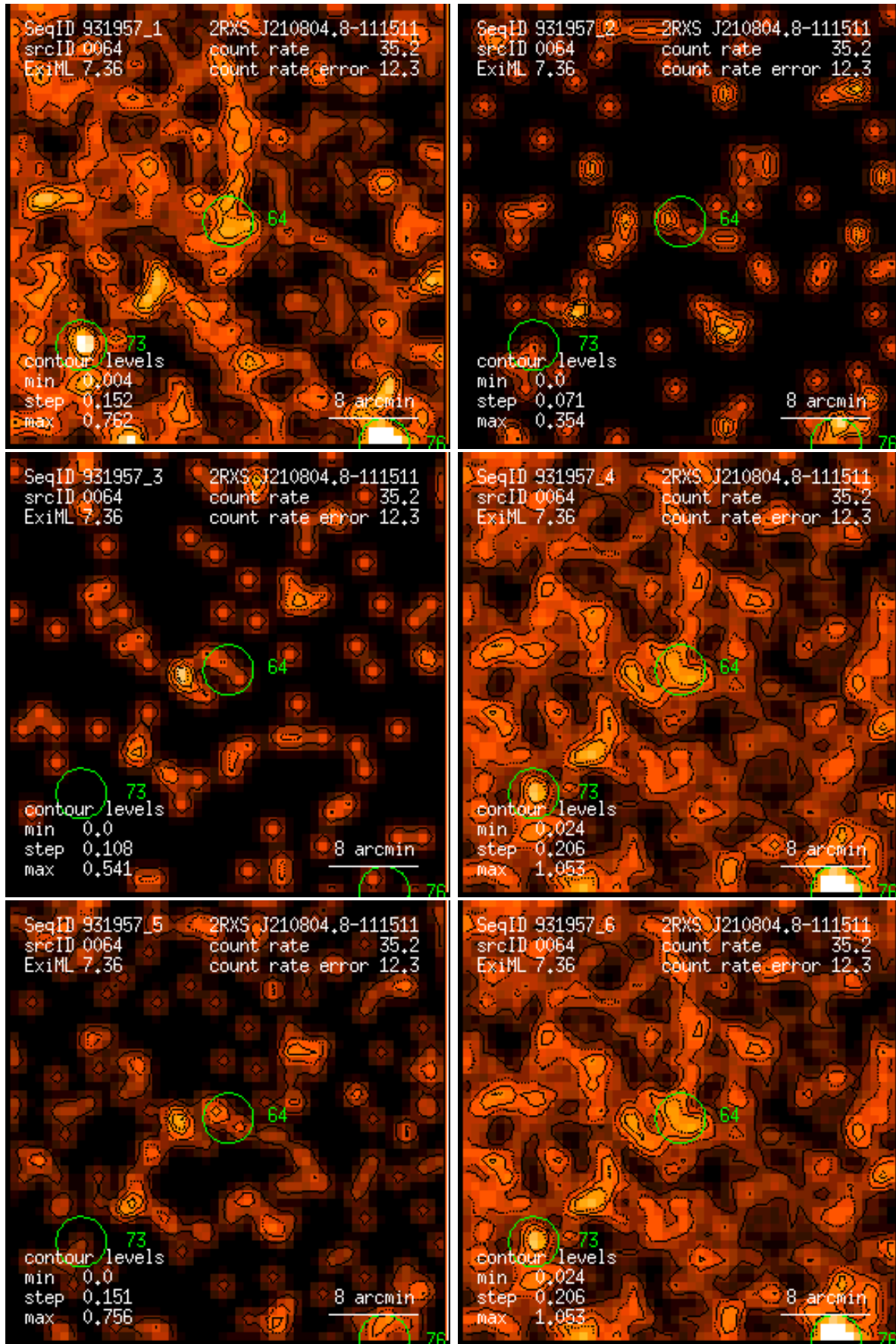
Figure 64: RASS 931957: detection 0064: band rate images, Gaussian filter: (1) PSPC channels 11 – 41, (2) 52 – 90, (3) 91 – 201, (4) 11 – 235, (5) 52 – 201, (6) 11 – 201. Broad band rates in counts/ks. Band rate contour levels in counts/ks/arcmin 2 .
