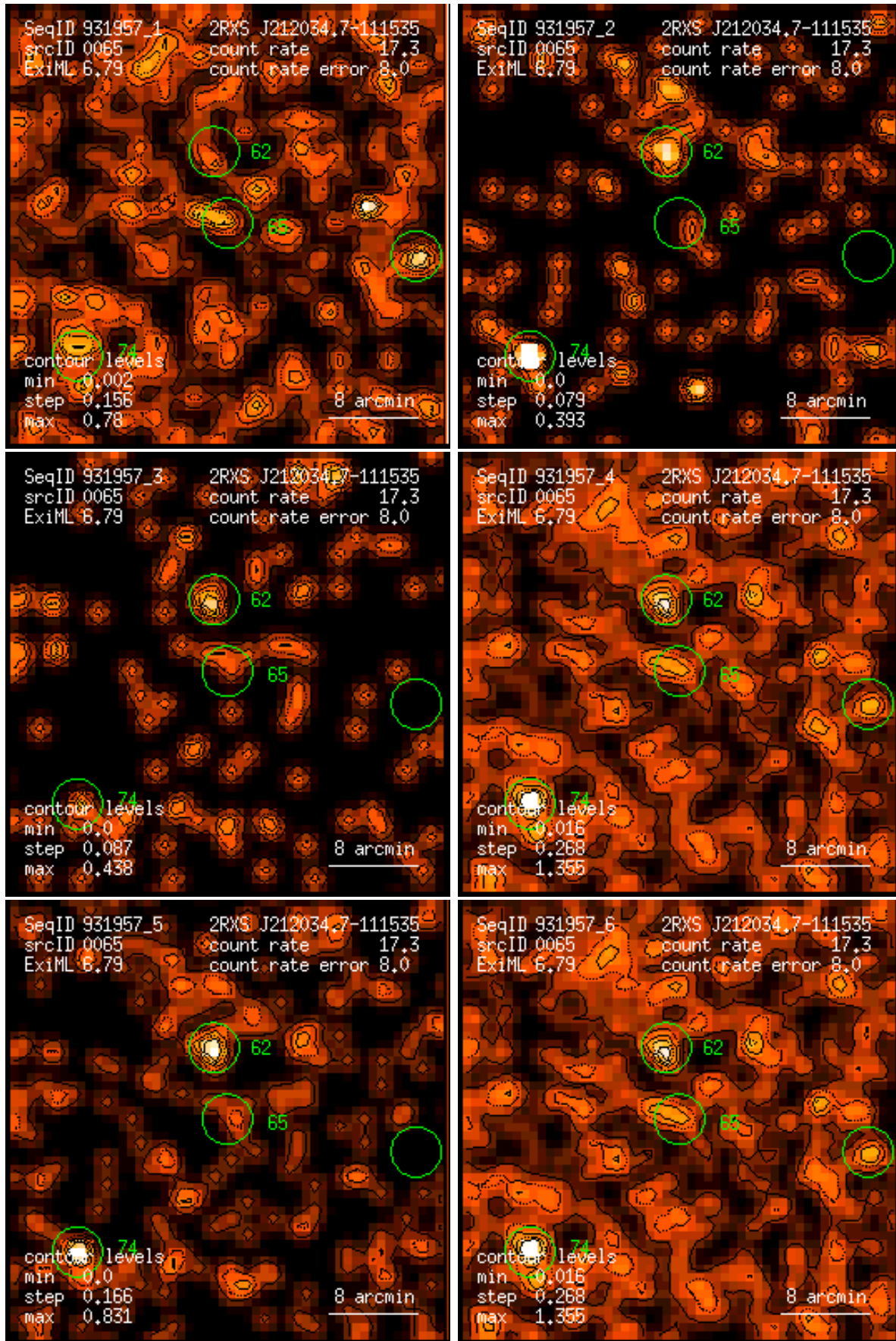
Figure 65: RASS 931957: detection 0065: band rate images, Gaussian filter: (1) PSPC channels 11 – 41, (2) 52 – 90, (3) 91 – 201, (4) 11 – 235, (5) 52 – 201, (6) 11 – 201. Broad band rates in counts/ks. Band rate contour levels in counts/ks/arcmin 2 .
