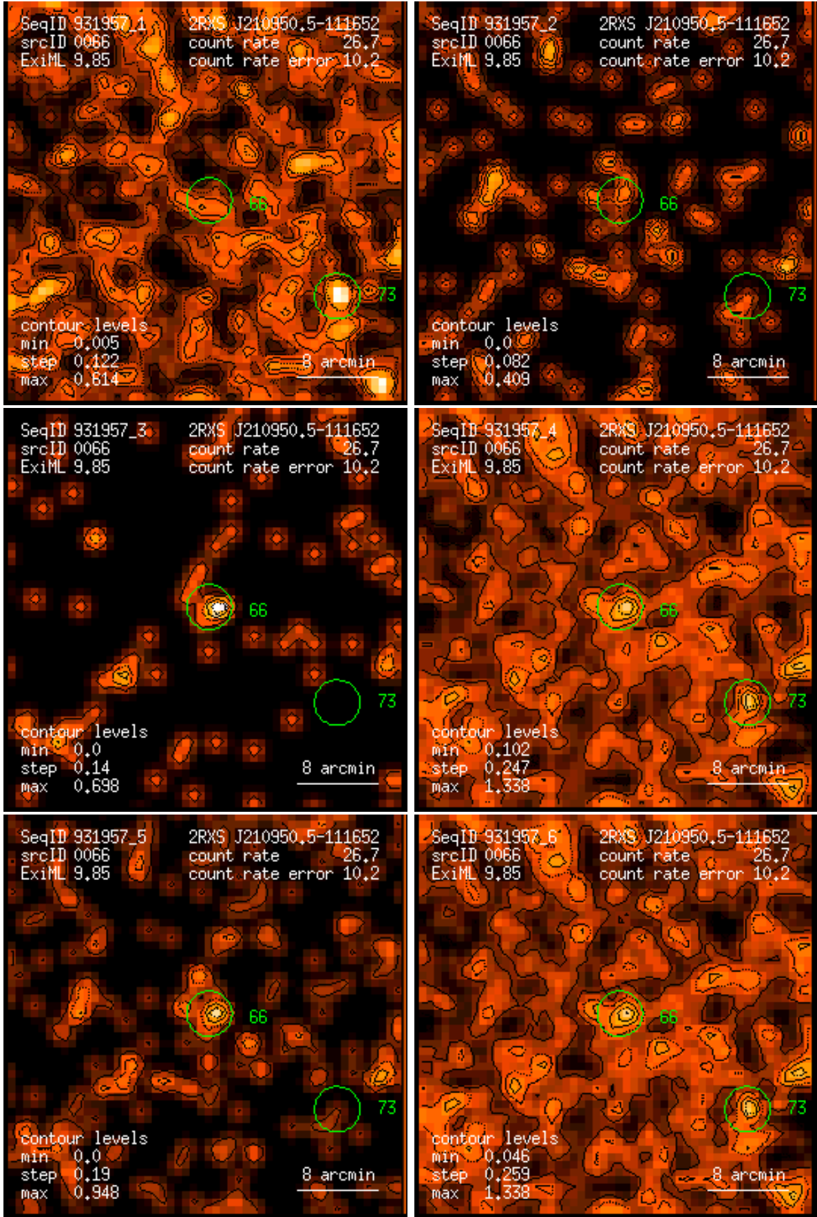
Figure 66: RASS 931957: detection 0066: band rate images, Gaussian filter: (1) PSPC channels 11 – 41, (2) 52 – 90, (3) 91 – 201, (4) 11 – 235, (5) 52 – 201, (6) 11 – 201. Broad band rates in counts/ks. Band rate contour levels in counts/ks/arcmin 2 .
