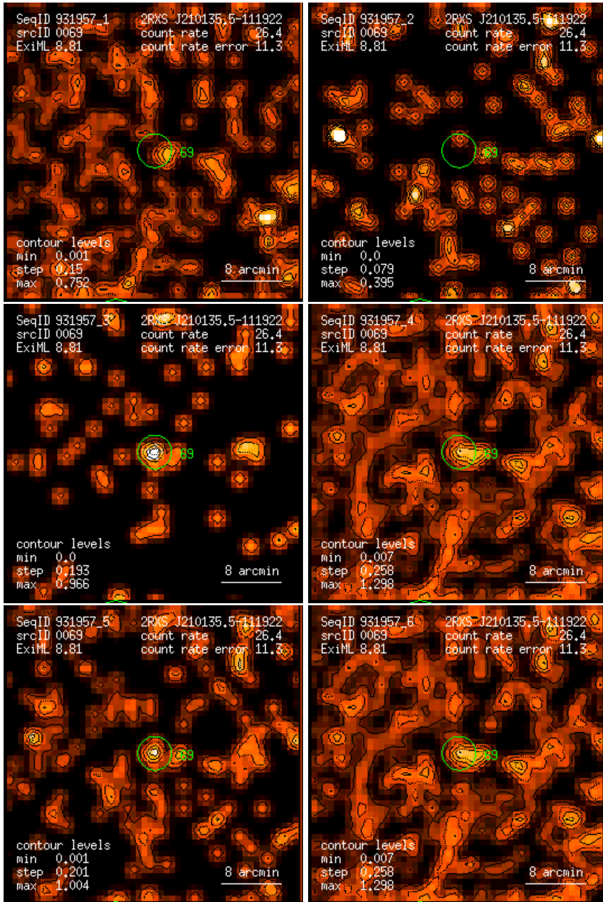
Figure 69: RASS 931957: detection 0069: band rate images, Gaussian filter: (1) PSPC channels 11 – 41, (2) 52 – 90, (3) 91 – 201, (4) 11 – 235, (5) 52 – 201, (6) 11 – 201. Broad band rates in counts/ks. Band rate contour levels in counts/ks/arcmin 2 .
