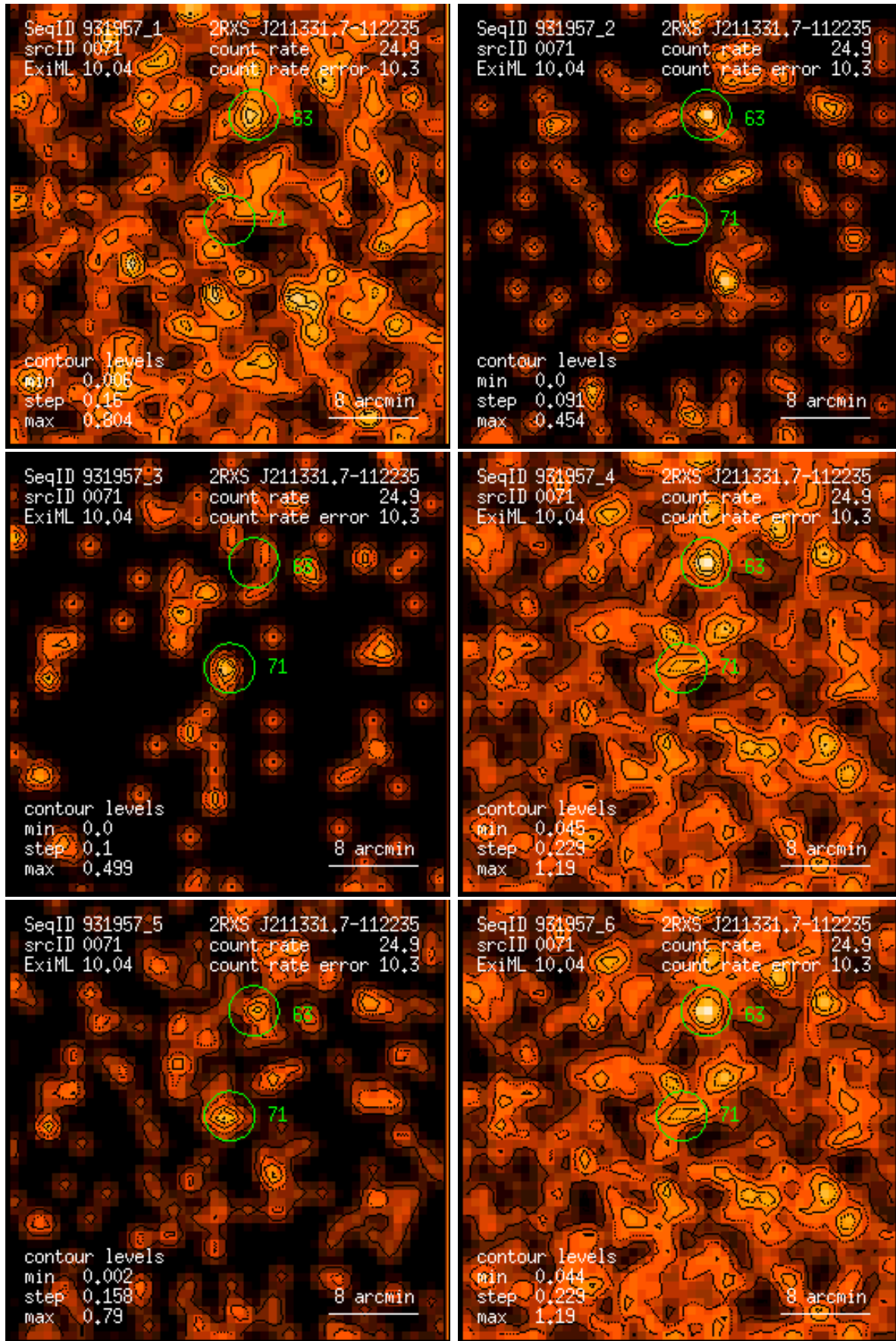
Figure 71: RASS 931957: detection 0071: band rate images, Gaussian filter: (1) PSPC channels 11 – 41, (2) 52 – 90, (3) 91 – 201, (4) 11 – 235, (5) 52 – 201, (6) 11 – 201. Broad band rates in counts/ks. Band rate contour levels in counts/ks/arcmin 2 .
