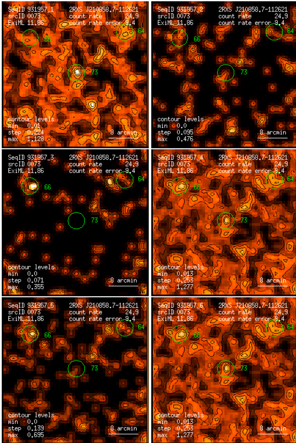
Figure 73: RASS 931957: detection 0073: band rate images, Gaussian filter: (1) PSPC channels 11 – 41, (2) 52 – 90, (3) 91 – 201, (4) 11 – 235, (5) 52 – 201, (6) 11 – 201. Broad band rates in counts/ks. Band rate contour levels in counts/ks/arcmin 2 .
