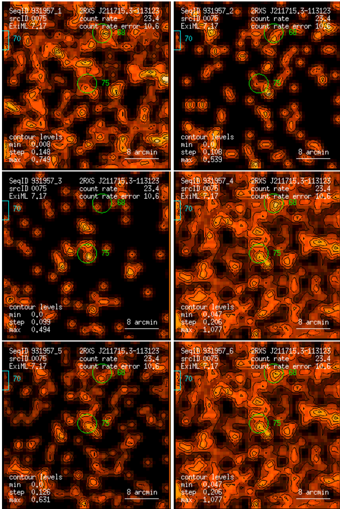
Figure 75: RASS 931957: detection 0075: band rate images, Gaussian filter: (1) PSPC channels 11 – 41, (2) 52 – 90, (3) 91 – 201, (4) 11 – 235, (5) 52 – 201, (6) 11 – 201. Broad band rates in counts/ks. Band rate contour levels in counts/ks/arcmin 2 .
