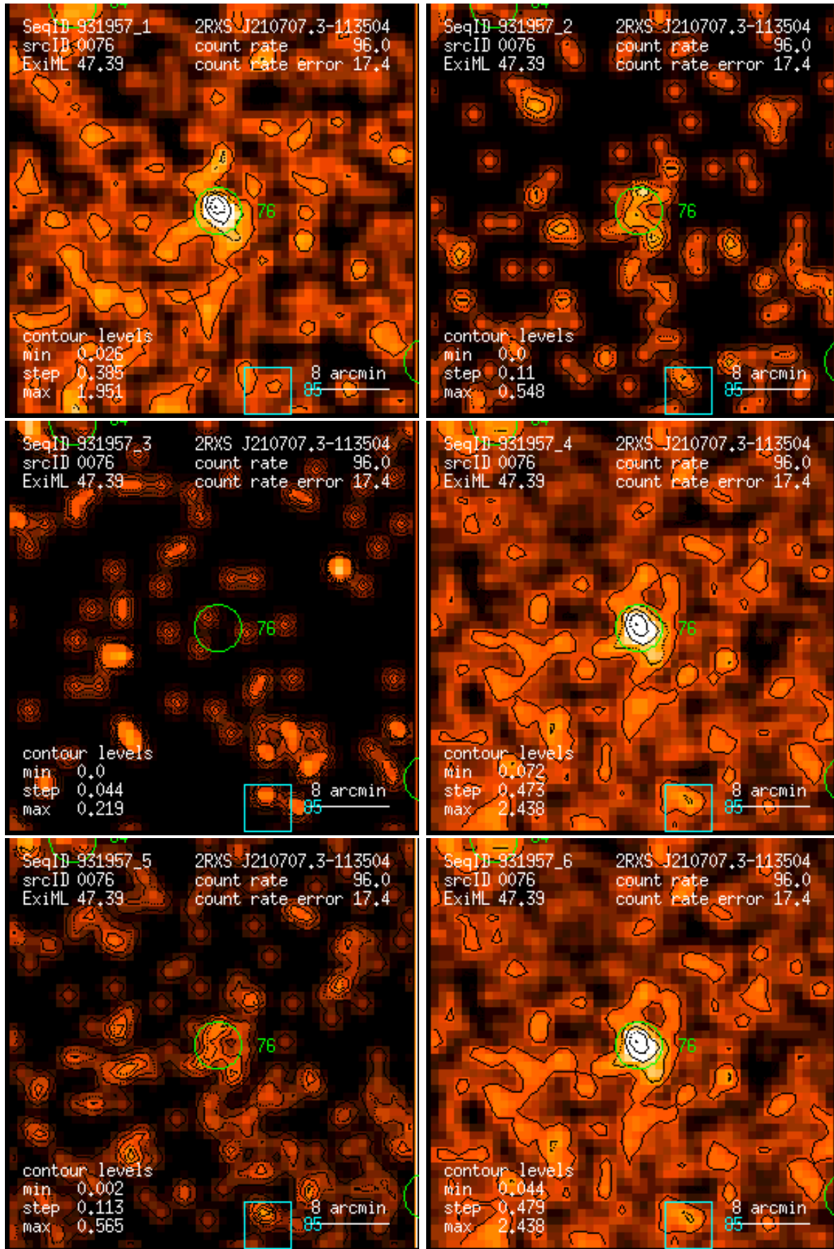
Figure 76: RASS 931957: detection 0076: band rate images, Gaussian filter: (1) PSPC channels 11 – 41, (2) 52 – 90, (3) 91 – 201, (4) 11 – 235, (5) 52 – 201, (6) 11 – 201. Broad band rates in counts/ks. Band rate contour levels in counts/ks/arcmin 2 .
