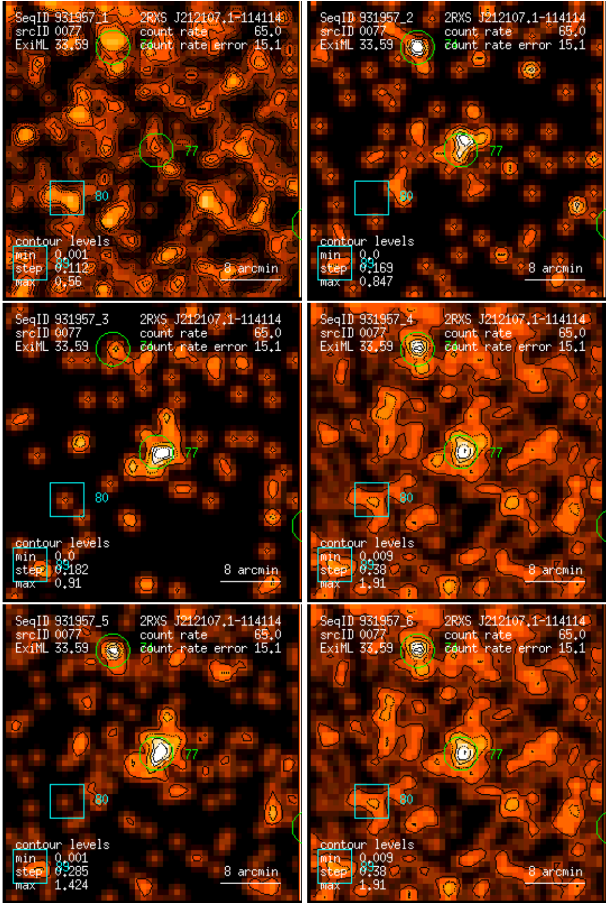
Figure 77: RASS 931957: detection 0077: band rate images, Gaussian filter: (1) PSPC channels 11 – 41, (2) 52 – 90, (3) 91 – 201, (4) 11 – 235, (5) 52 – 201, (6) 11 – 201. Broad band rates in counts/ks. Band rate contour levels in counts/ks/arcmin 2 .
