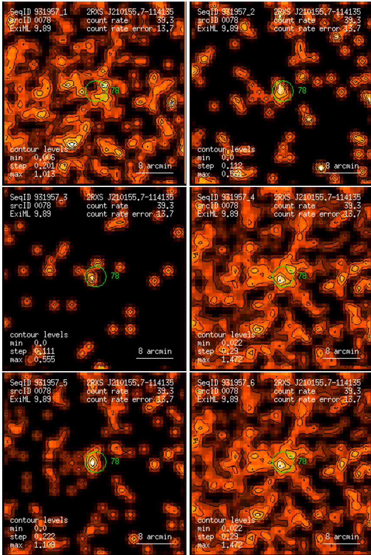
Figure 78: RASS 931957: detection 0078: band rate images, Gaussian filter: (1) PSPC channels 11 – 41, (2) 52 – 90, (3) 91 – 201, (4) 11 – 235, (5) 52 – 201, (6) 11 – 201. Broad band rates in counts/ks. Band rate contour levels in counts/ks/arcmin 2 .
