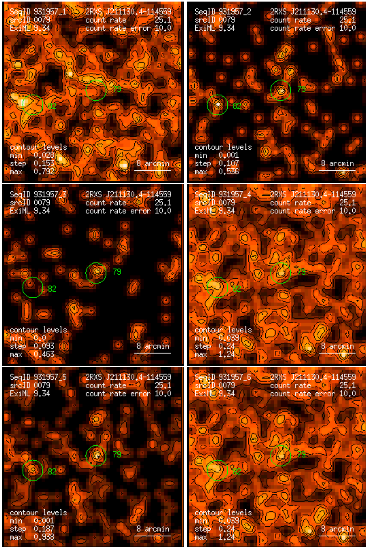
Figure 79: RASS 931957: detection 0079: band rate images, Gaussian filter: (1) PSPC channels 11 – 41, (2) 52 – 90, (3) 91 – 201, (4) 11 – 235, (5) 52 – 201, (6) 11 – 201. Broad band rates in counts/ks. Band rate contour levels in counts/ks/arcmin 2 .
