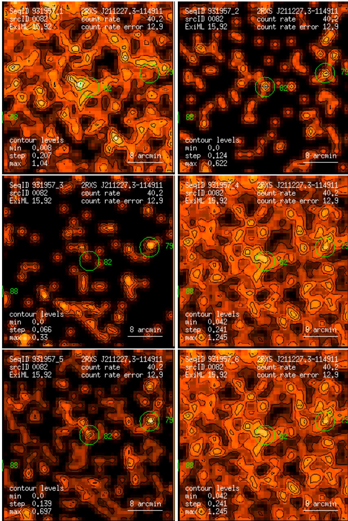
Figure 82: RASS 931957: detection 0082: band rate images, Gaussian filter: (1) PSPC channels 11 – 41, (2) 52 – 90, (3) 91 – 201, (4) 11 – 235, (5) 52 – 201, (6) 11 – 201. Broad band rates in counts/ks. Band rate contour levels in counts/ks/arcmin 2 .
