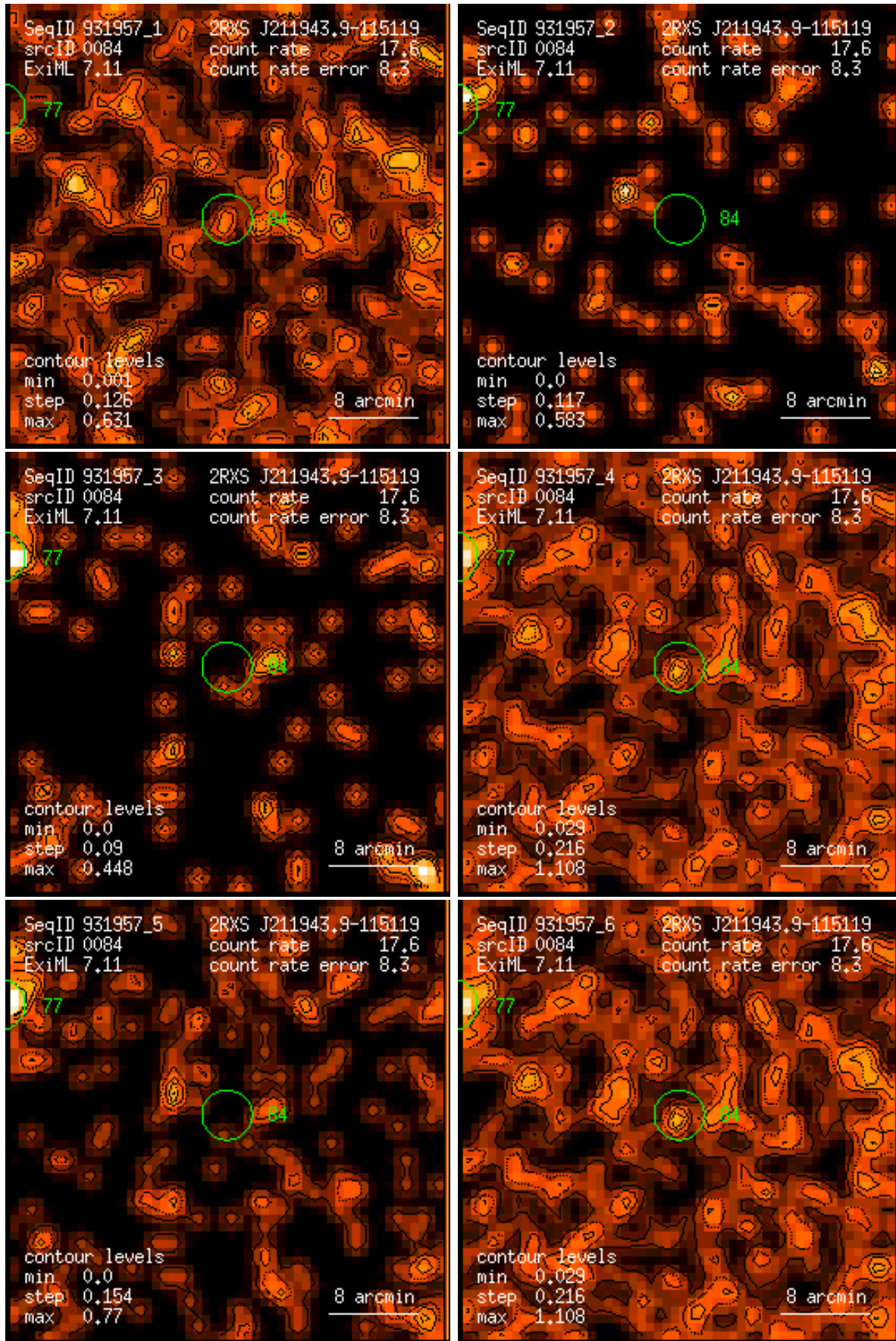
Figure 84: RASS 931957: detection 0084: band rate images, Gaussian filter: (1) PSPC channels 11 – 41, (2) 52 – 90, (3) 91 – 201, (4) 11 – 235, (5) 52 – 201, (6) 11 – 201. Broad band rates in counts/ks. Band rate contour levels in counts/ks/arcmin 2 .
