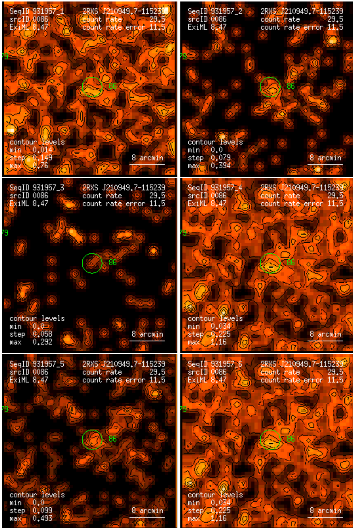
Figure 86: RASS 931957: detection 0086: band rate images, Gaussian filter: (1) PSPC channels 11 – 41, (2) 52 – 90, (3) 91 – 201, (4) 11 – 235, (5) 52 – 201, (6) 11 – 201. Broad band rates in counts/ks. Band rate contour levels in counts/ks/arcmin 2 .
