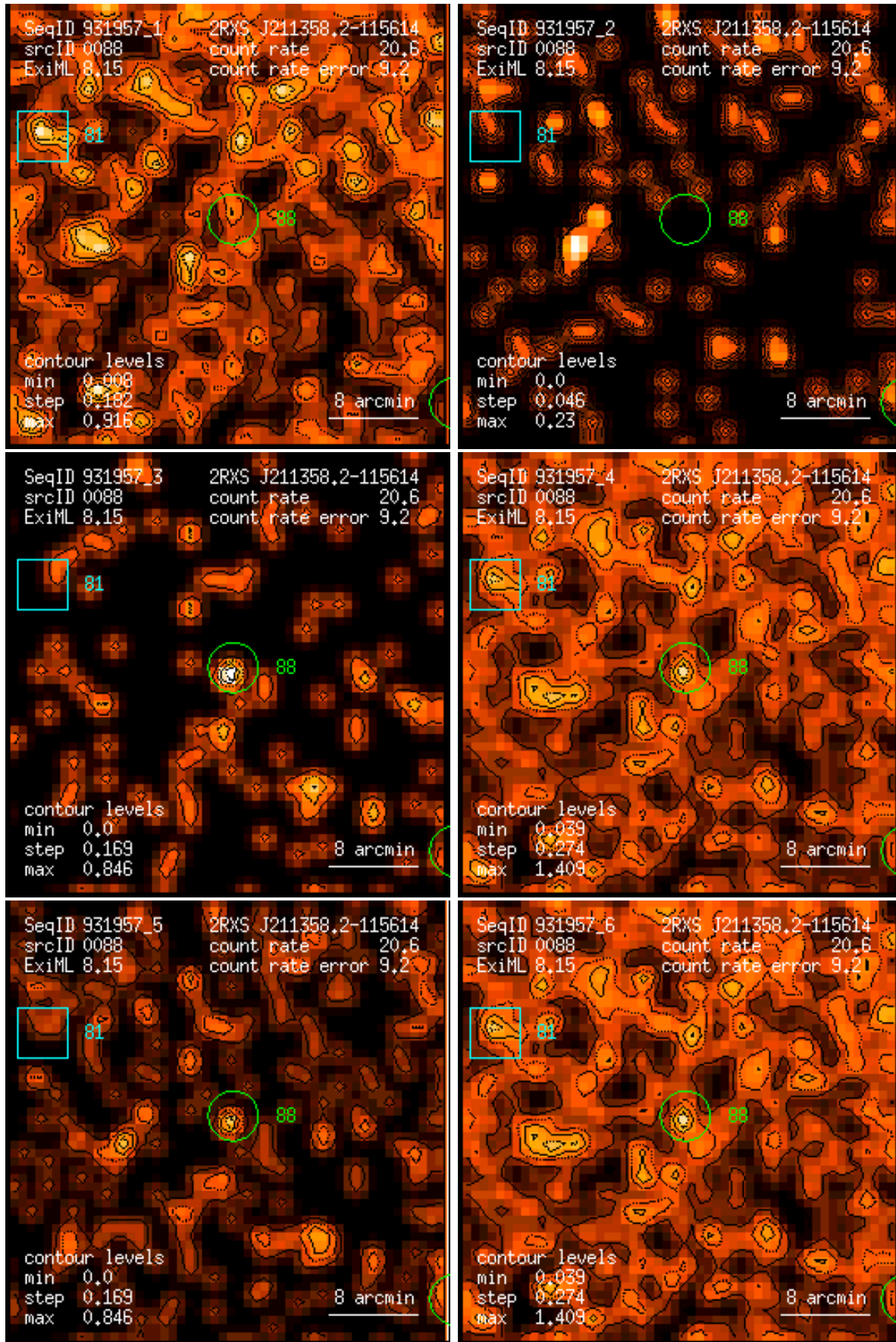
Figure 88: RASS 931957: detection 0088: band rate images, Gaussian filter: (1) PSPC channels 11 – 41, (2) 52 – 90, (3) 91 – 201, (4) 11 – 235, (5) 52 – 201, (6) 11 – 201. Broad band rates in counts/ks. Band rate contour levels in counts/ks/arcmin 2 .
