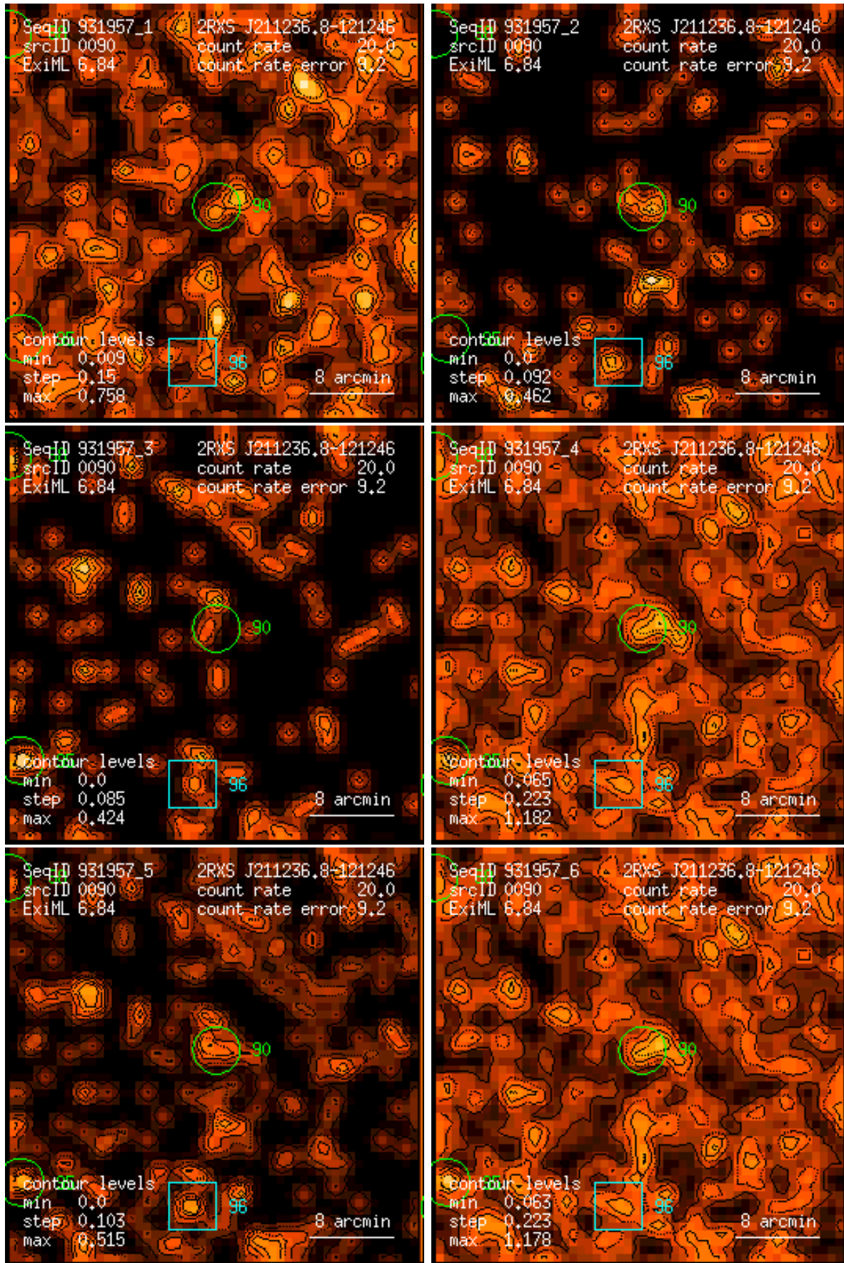
Figure 90: RASS 931957: detection 0090: band rate images, Gaussian filter: (1) PSPC channels 11 – 41, (2) 52 – 90, (3) 91 – 201, (4) 11 – 235, (5) 52 – 201, (6) 11 – 201. Broad band rates in counts/ks. Band rate contour levels in counts/ks/arcmin 2 .
