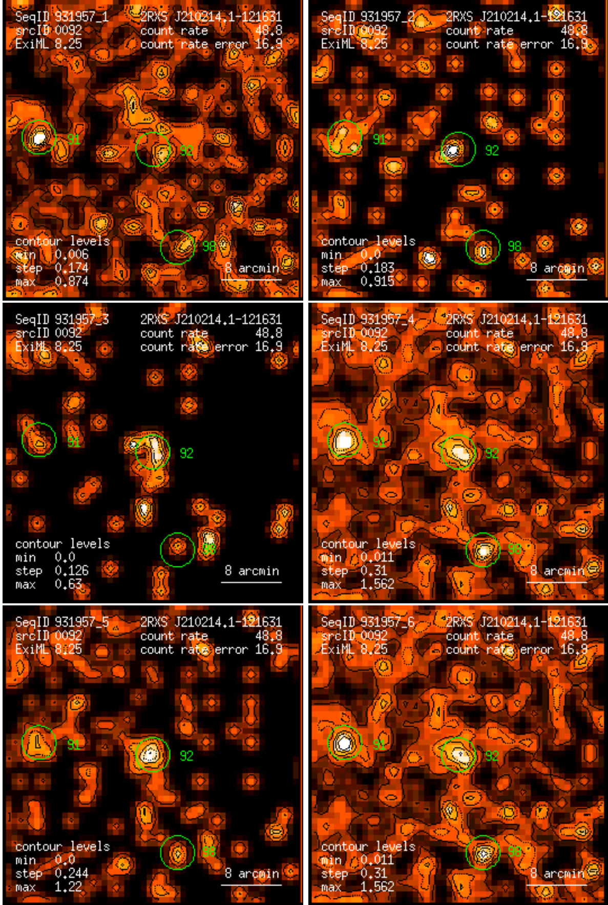
Figure 92: RASS 931957: detection 0092: band rate images, Gaussian filter: (1) PSPC channels 11 – 41, (2) 52 – 90, (3) 91 – 201, (4) 11 – 235, (5) 52 – 201, (6) 11 – 201. Broad band rates in counts/ks. Band rate contour levels in counts/ks/arcmin 2 .
