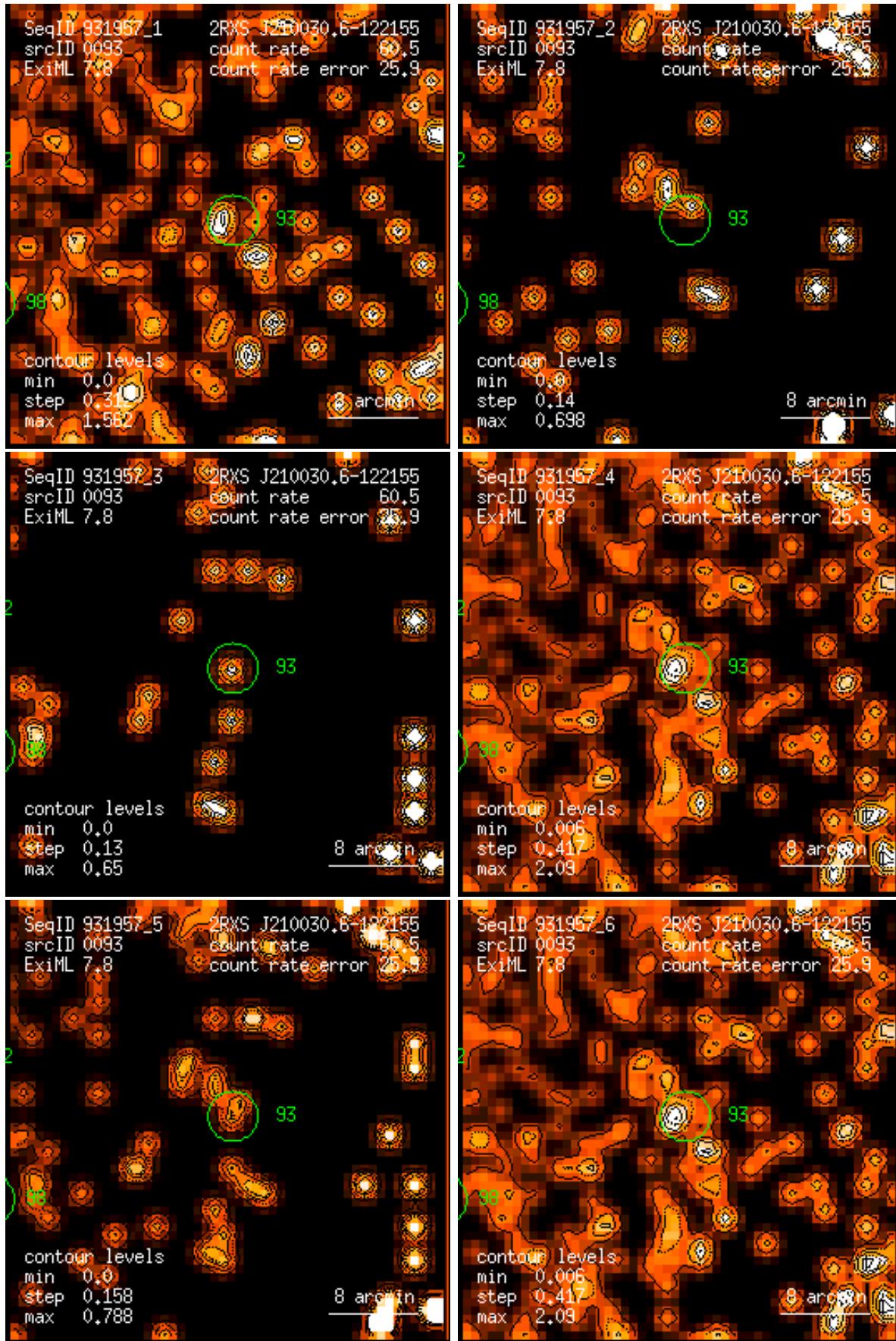
Figure 93: RASS 931957: detection 0093: band rate images, Gaussian filter: (1) PSPC channels 11 – 41, (2) 52 – 90, (3) 91 – 201, (4) 11 – 235, (5) 52 – 201, (6) 11 – 201. Broad band rates in counts/ks. Band rate contour levels in counts/ks/arcmin 2 .
