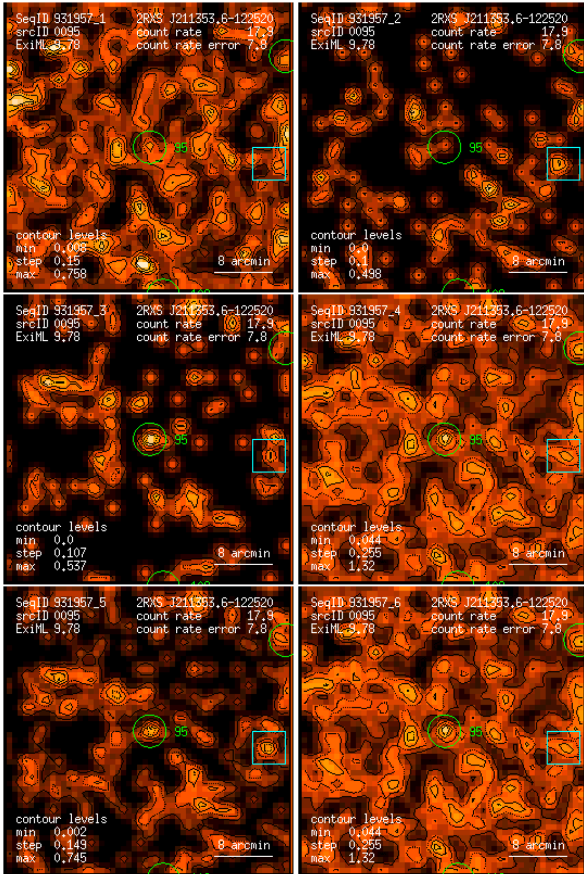
Figure 95: RASS 931957: detection 0095: band rate images, Gaussian filter: (1) PSPC channels 11 – 41, (2) 52 – 90, (3) 91 – 201, (4) 11 – 235, (5) 52 – 201, (6) 11 – 201. Broad band rates in counts/ks. Band rate contour levels in counts/ks/arcmin 2 .
