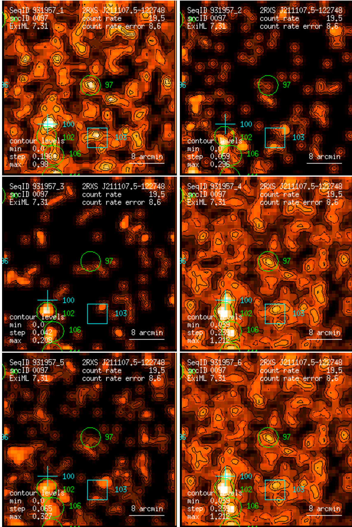
Figure 97: RASS 931957: detection 0097: band rate images, Gaussian filter: (1) PSPC channels 11 – 41, (2) 52 – 90, (3) 91 – 201, (4) 11 – 235, (5) 52 – 201, (6) 11 – 201. Broad band rates in counts/ks. Band rate contour levels in counts/ks/arcmin 2 .
