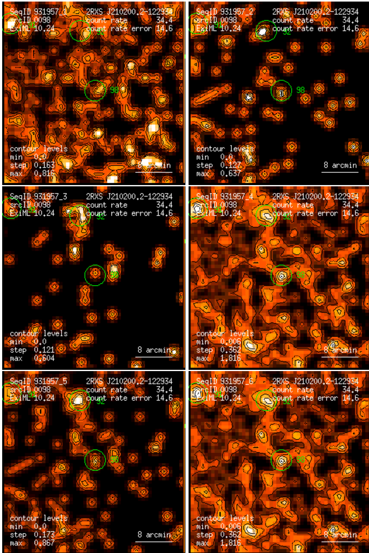
Figure 98: RASS 931957: detection 0098: band rate images, Gaussian filter: (1) PSPC channels 11 – 41, (2) 52 – 90, (3) 91 – 201, (4) 11 – 235, (5) 52 – 201, (6) 11 – 201. Broad band rates in counts/ks. Band rate contour levels in counts/ks/arcmin 2 .
