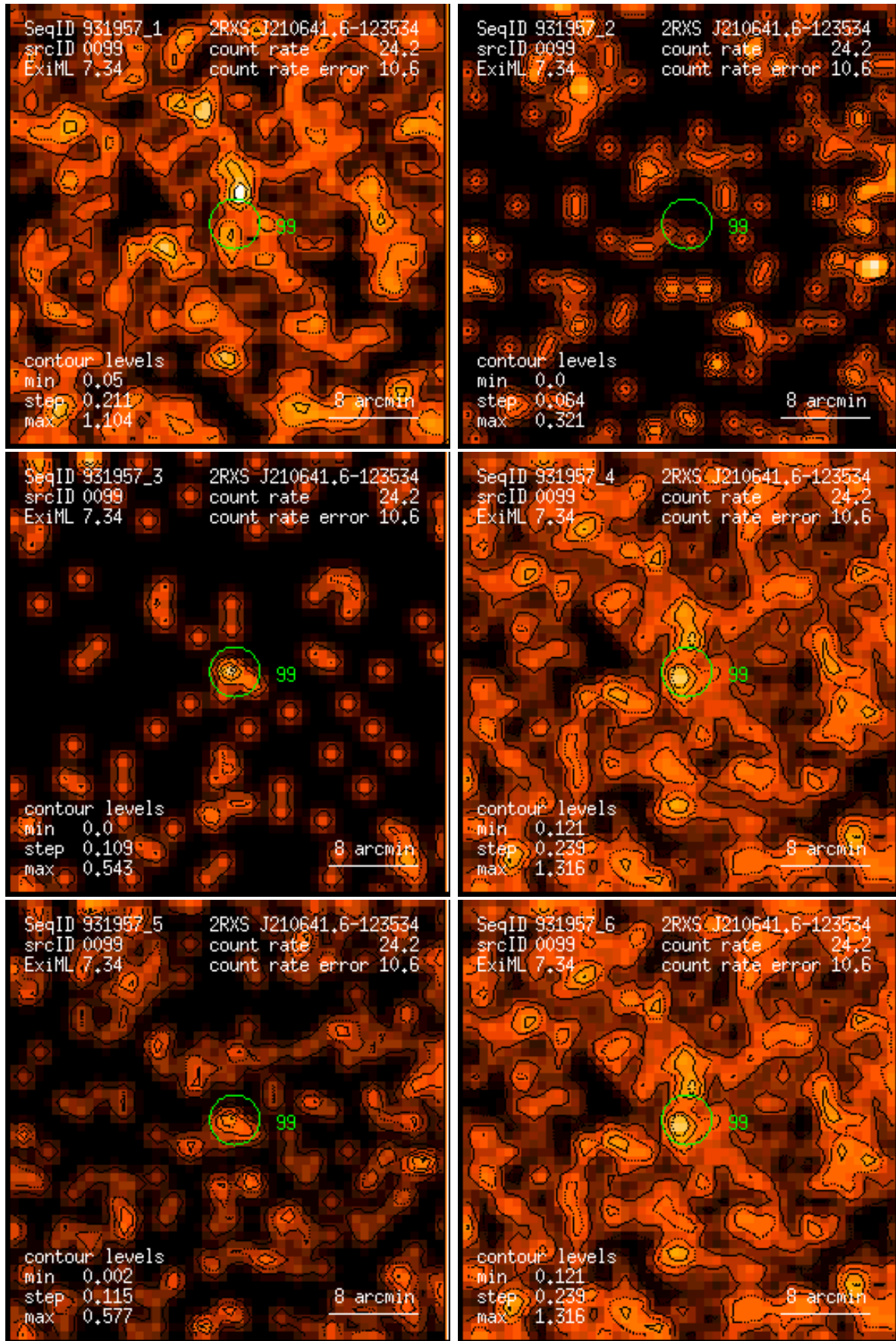
Figure 99: RASS 931957: detection 0099: band rate images, Gaussian filter: (1) PSPC channels 11 – 41, (2) 52 – 90, (3) 91 – 201, (4) 11 – 235, (5) 52 – 201, (6) 11 – 201. Broad band rates in counts/ks. Band rate contour levels in counts/ks/arcmin 2 .
