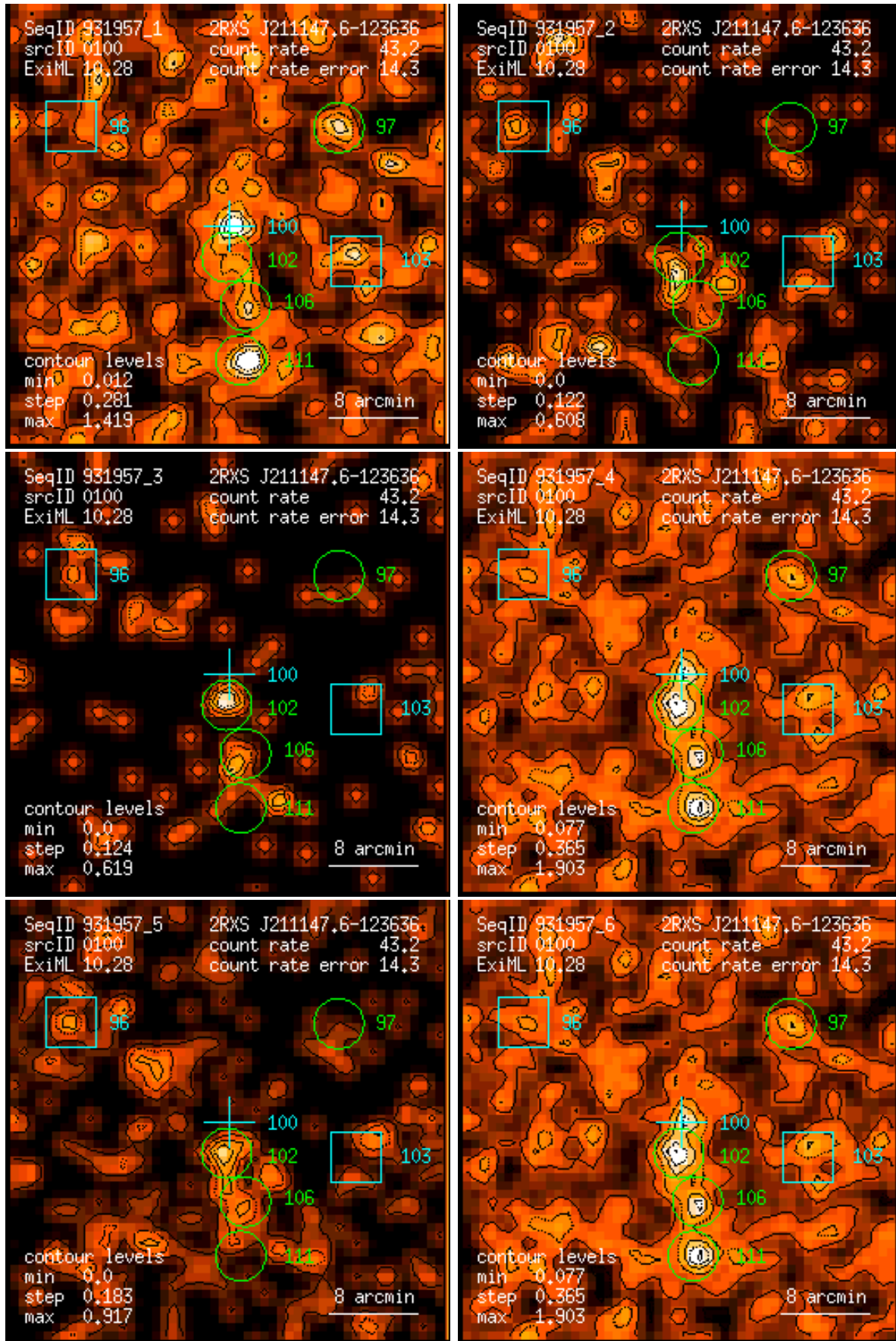
Figure 100: RASS 931957: detection 0100: band rate images, Gaussian filter: (1) PSPC channels 11 – 41, (2) 52 – 90, (3) 91 – 201, (4) 11 – 235, (5) 52 – 201, (6) 11 – 201. Broad band rates in counts/ks. Band rate contour levels in counts/ks/arcmin 2 .
