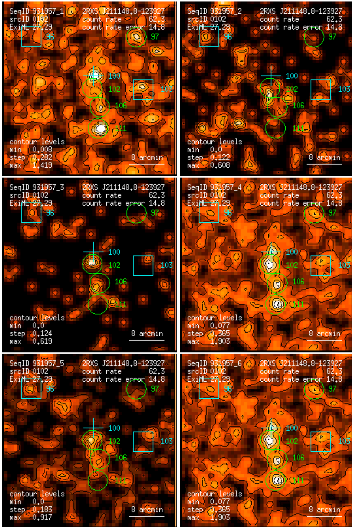
Figure 102: RASS 931957: detection 0102: band rate images, Gaussian filter: (1) PSPC channels 11 – 41, (2) 52 – 90, (3) 91 – 201, (4) 11 – 235, (5) 52 – 201, (6) 11 – 201. Broad band rates in counts/ks. Band rate contour levels in counts/ks/arcmin 2 .
