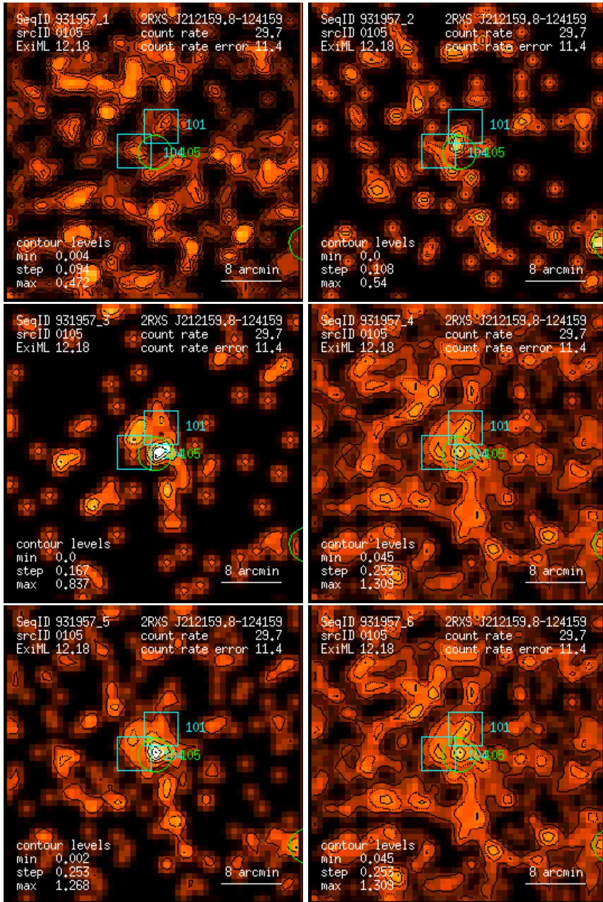
Figure 105: RASS 931957: detection 0105: band rate images, Gaussian filter: (1) PSPC channels 11 – 41, (2) 52 – 90, (3) 91 – 201, (4) 11 – 235, (5) 52 – 201, (6) 11 – 201. Broad band rates in counts/ks. Band rate contour levels in counts/ks/arcmin 2 .
