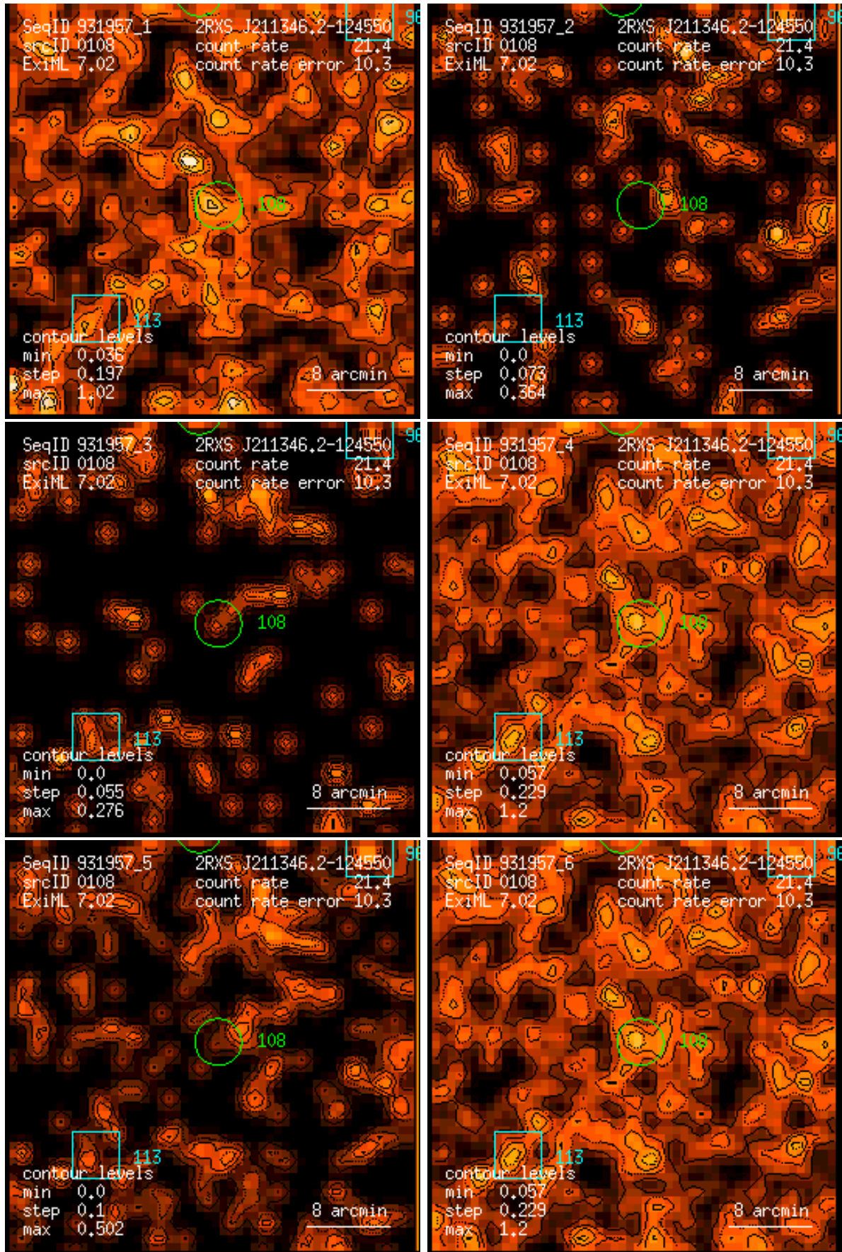
Figure 108: RASS 931957: detection 0108: band rate images, Gaussian filter: (1) PSPC channels 11 – 41, (2) 52 – 90, (3) 91 – 201, (4) 11 – 235, (5) 52 – 201, (6) 11 – 201. Broad band rates in counts/ks. Band rate contour levels in counts/ks/arcmin 2 .
