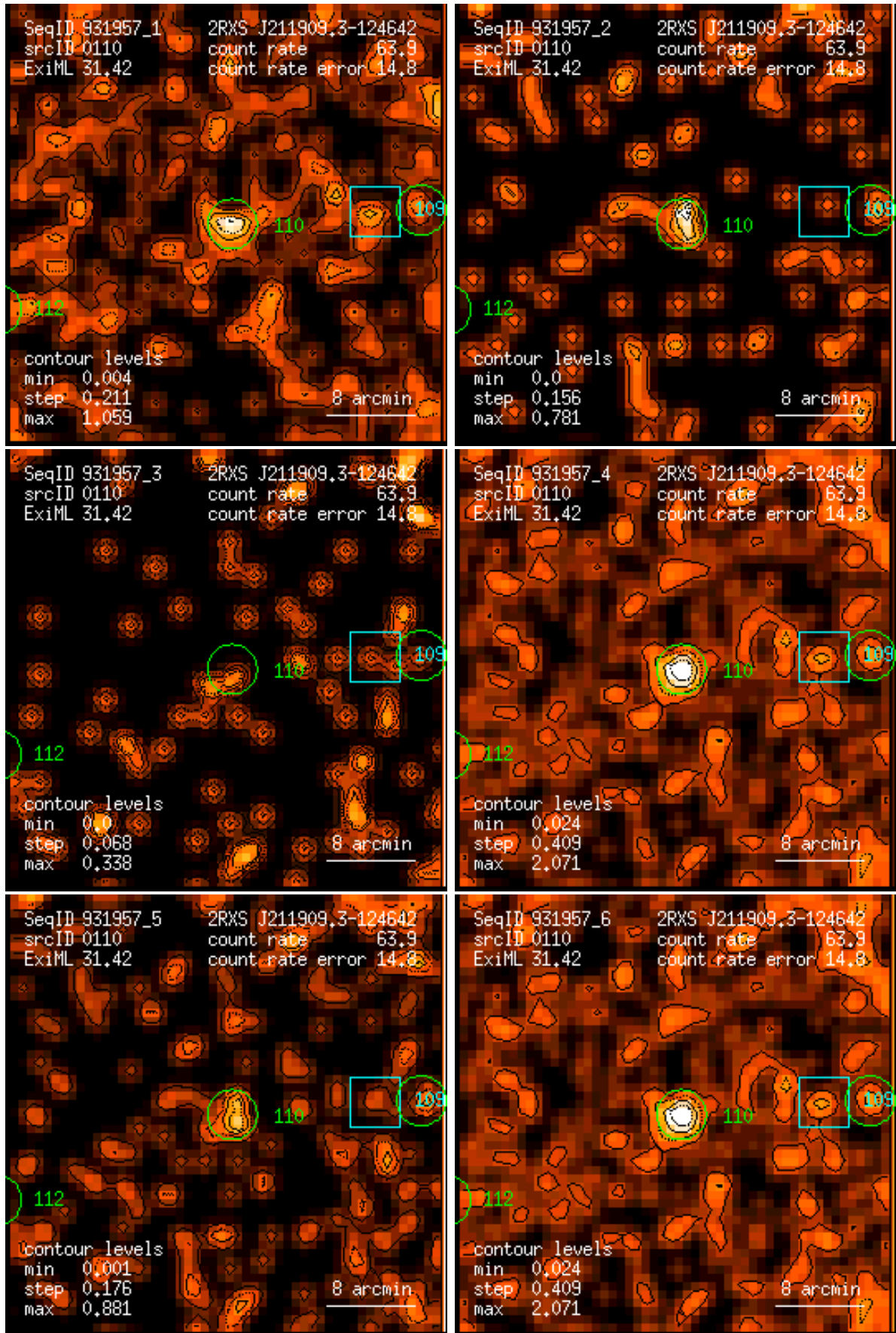
Figure 110: RASS 931957: detection 0110: band rate images, Gaussian filter: (1) PSPC channels 11 – 41, (2) 52 – 90, (3) 91 – 201, (4) 11 – 235, (5) 52 – 201, (6) 11 – 201. Broad band rates in counts/ks. Band rate contour levels in counts/ks/arcmin 2 .
