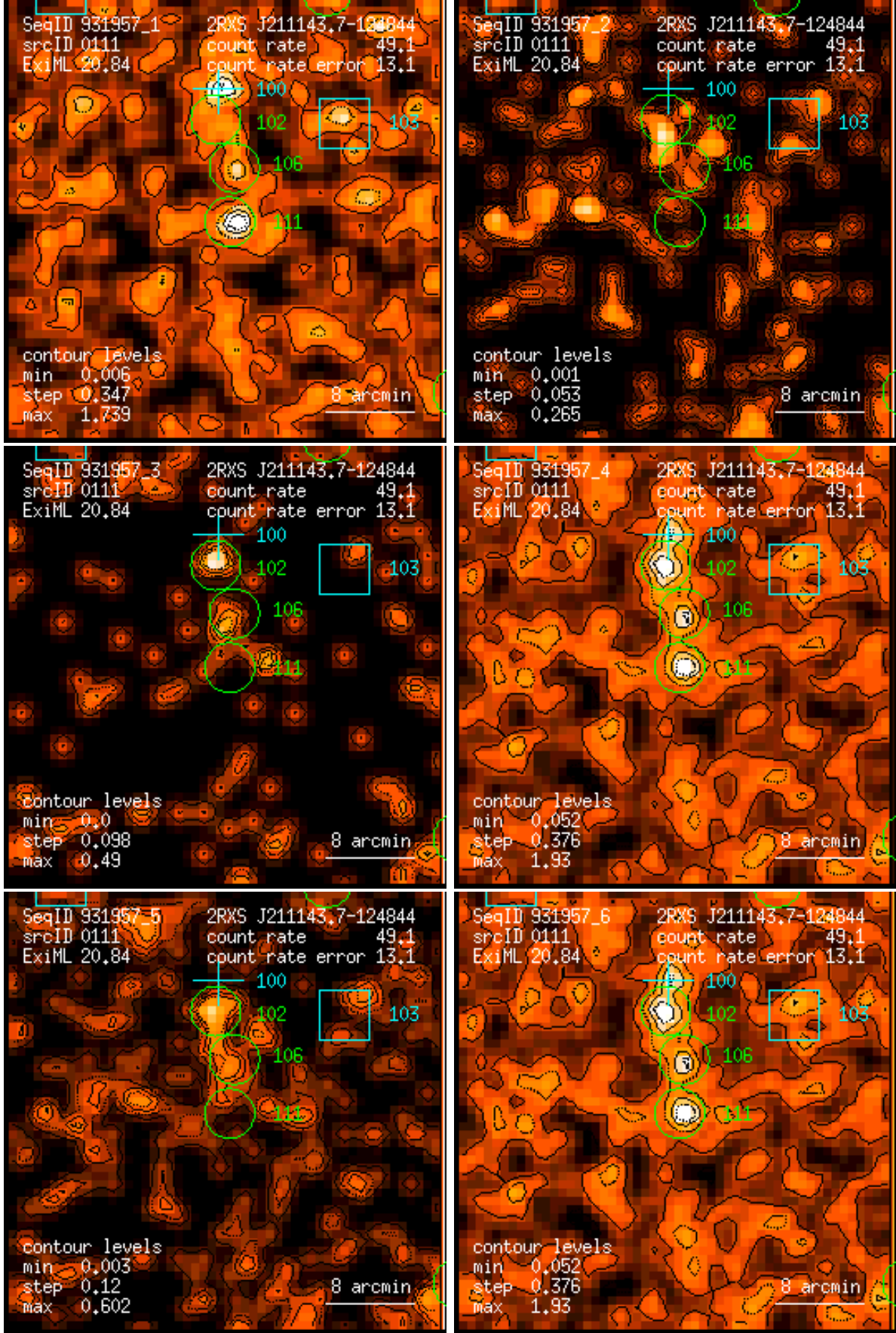
Figure 111: RASS 931957: detection 0111: band rate images, Gaussian filter: (1) PSPC channels 11 – 41, (2) 52 – 90, (3) 91 – 201, (4) 11 – 235, (5) 52 – 201, (6) 11 – 201. Broad band rates in counts/ks. Band rate contour levels in counts/ks/arcmin 2 .
