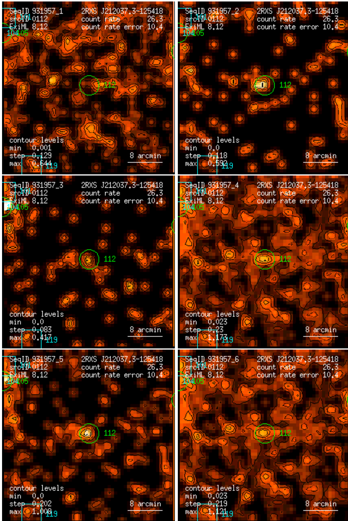
Figure 112: RASS 931957: detection 0112: band rate images, Gaussian filter: (1) PSPC channels 11 – 41, (2) 52 – 90, (3) 91 – 201, (4) 11 – 235, (5) 52 – 201, (6) 11 – 201. Broad band rates in counts/ks. Band rate contour levels in counts/ks/arcmin 2 .
