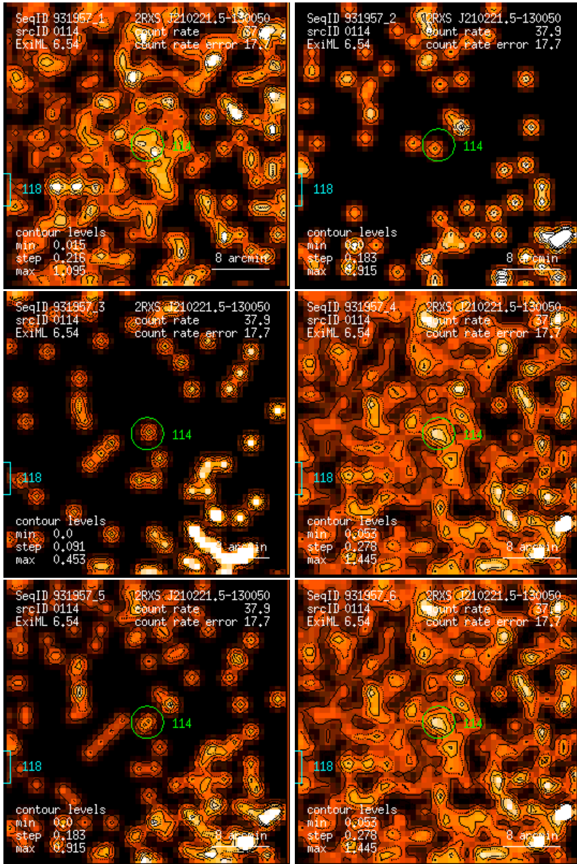
Figure 114: RASS 931957: detection 0114: band rate images, Gaussian filter: (1) PSPC channels 11 – 41, (2) 52 – 90, (3) 91 – 201, (4) 11 – 235, (5) 52 – 201, (6) 11 – 201. Broad band rates in counts/ks. Band rate contour levels in counts/ks/arcmin 2 .
