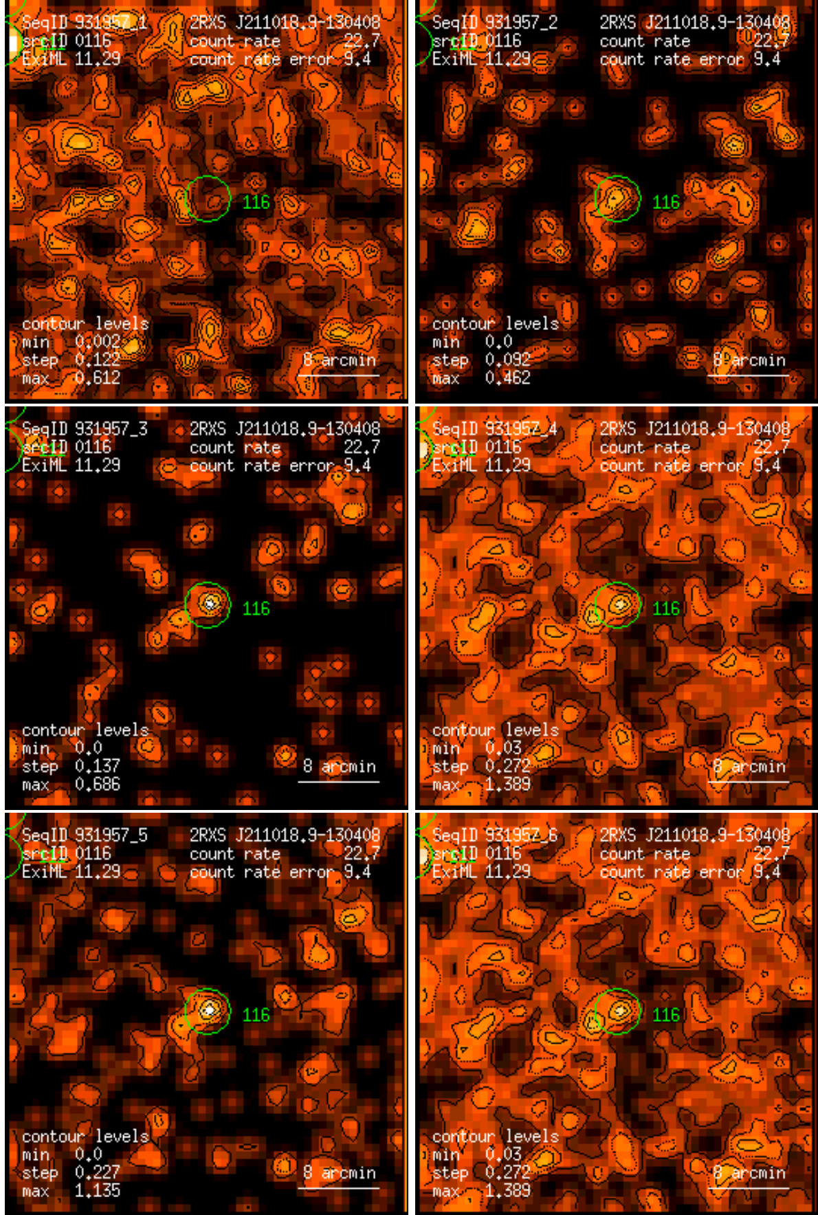
Figure 116: RASS 931957: detection 0116: band rate images, Gaussian filter: (1) PSPC channels 11 – 41, (2) 52 – 90, (3) 91 – 201, (4) 11 – 235, (5) 52 – 201, (6) 11 – 201. Broad band rates in counts/ks. Band rate contour levels in counts/ks/arcmin 2 .
