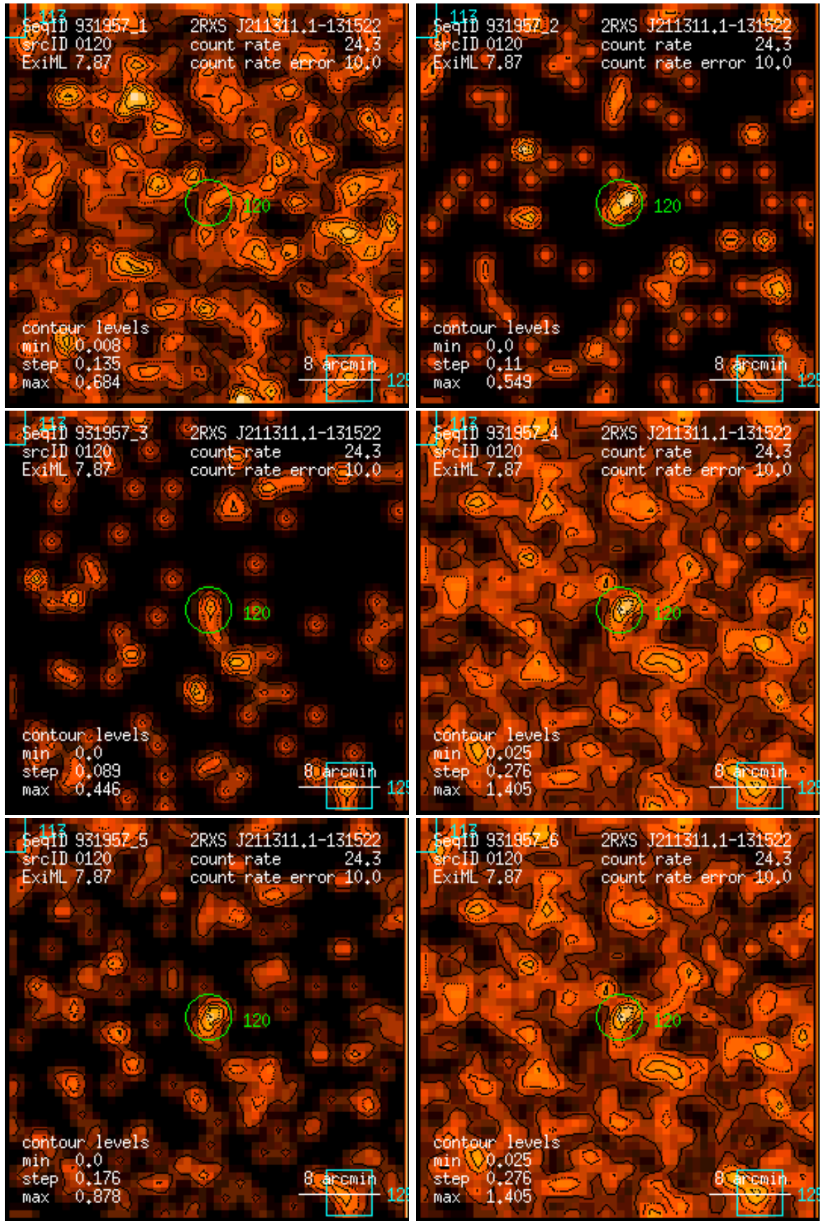
Figure 120: RASS 931957: detection 0120: band rate images, Gaussian filter: (1) PSPC channels 11 – 41, (2) 52 – 90, (3) 91 – 201, (4) 11 – 235, (5) 52 – 201, (6) 11 – 201. Broad band rates in counts/ks. Band rate contour levels in counts/ks/arcmin 2 .
