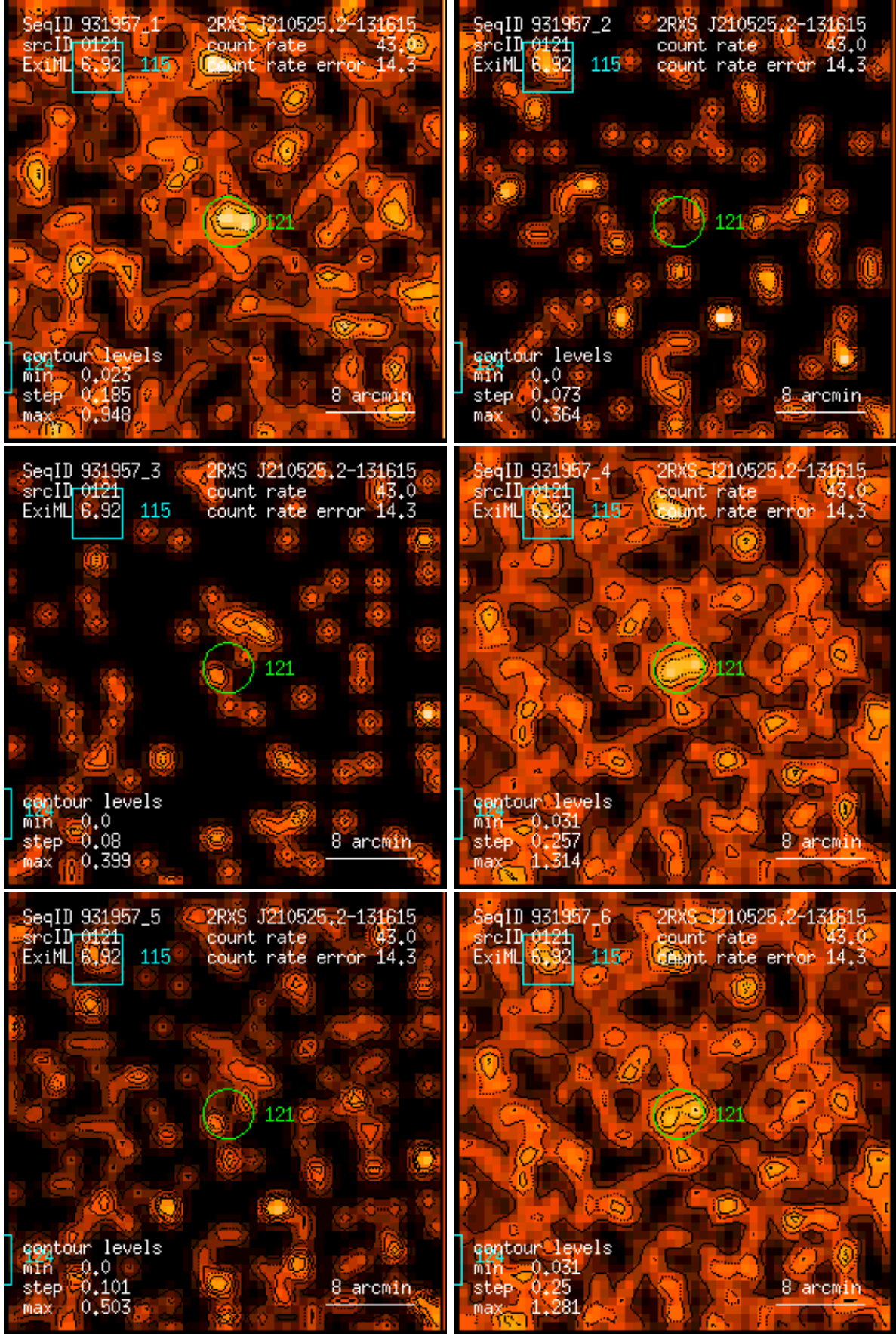
Figure 121: RASS 931957: detection 0121: band rate images, Gaussian filter: (1) PSPC channels 11 – 41, (2) 52 – 90, (3) 91 – 201, (4) 11 – 235, (5) 52 – 201, (6) 11 – 201. Broad band rates in counts/ks. Band rate contour levels in counts/ks/arcmin 2 .
