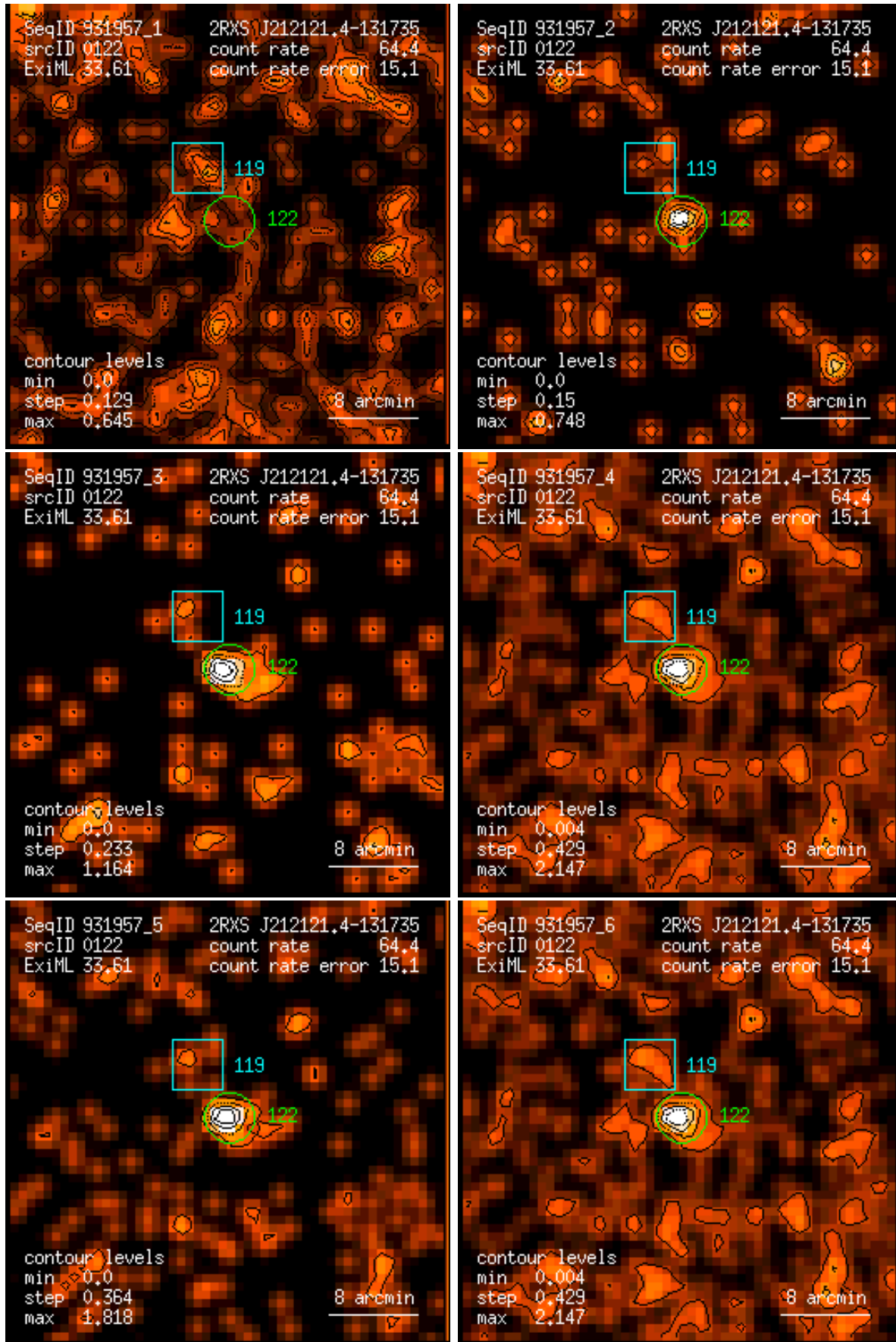
Figure 122: RASS 931957: detection 0122: band rate images, Gaussian filter: (1) PSPC channels 11 – 41, (2) 52 – 90, (3) 91 – 201, (4) 11 – 235, (5) 52 – 201, (6) 11 – 201. Broad band rates in counts/ks. Band rate contour levels in counts/ks/arcmin 2 .
