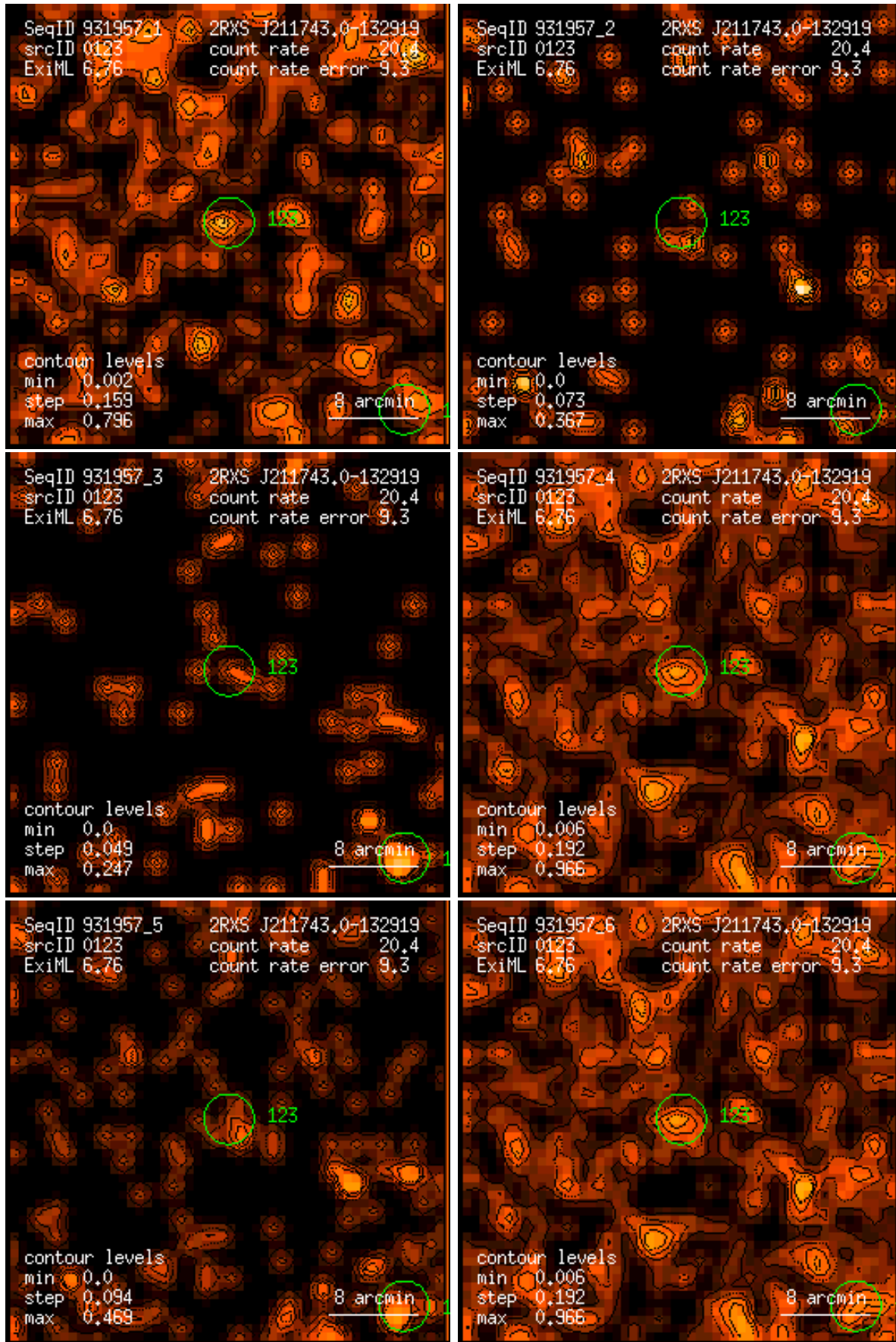
Figure 123: RASS 931957: detection 0123: band rate images, Gaussian filter: (1) PSPC channels 11 – 41, (2) 52 – 90, (3) 91 – 201, (4) 11 – 235, (5) 52 – 201, (6) 11 – 201. Broad band rates in counts/ks. Band rate contour levels in counts/ks/arcmin 2 .
