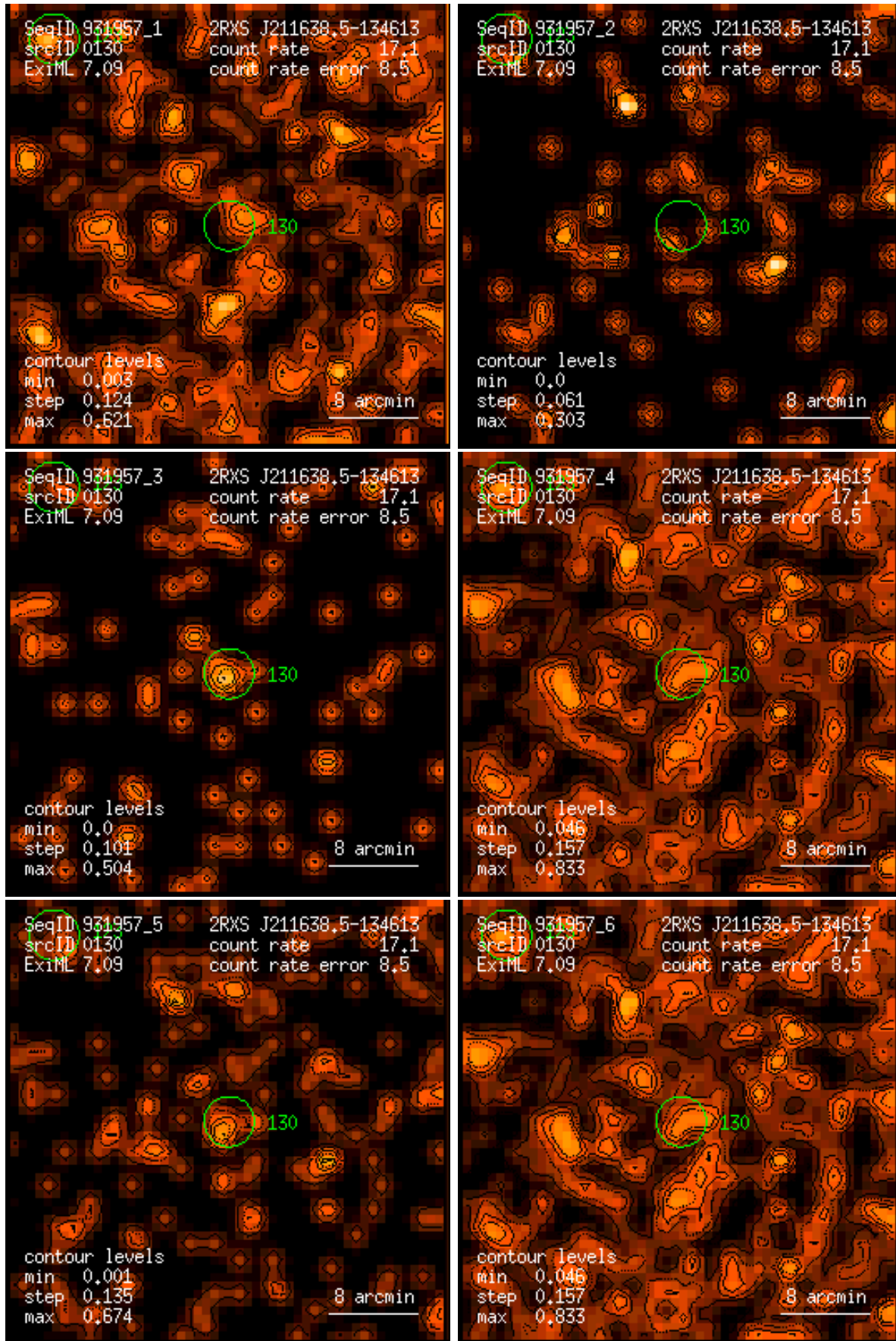
Figure 130: RASS 931957: detection 0130: band rate images, Gaussian filter: (1) PSPC channels 11 – 41, (2) 52 – 90, (3) 91 – 201, (4) 11 – 235, (5) 52 – 201, (6) 11 – 201. Broad band rates in counts/ks. Band rate contour levels in counts/ks/arcmin 2 .
