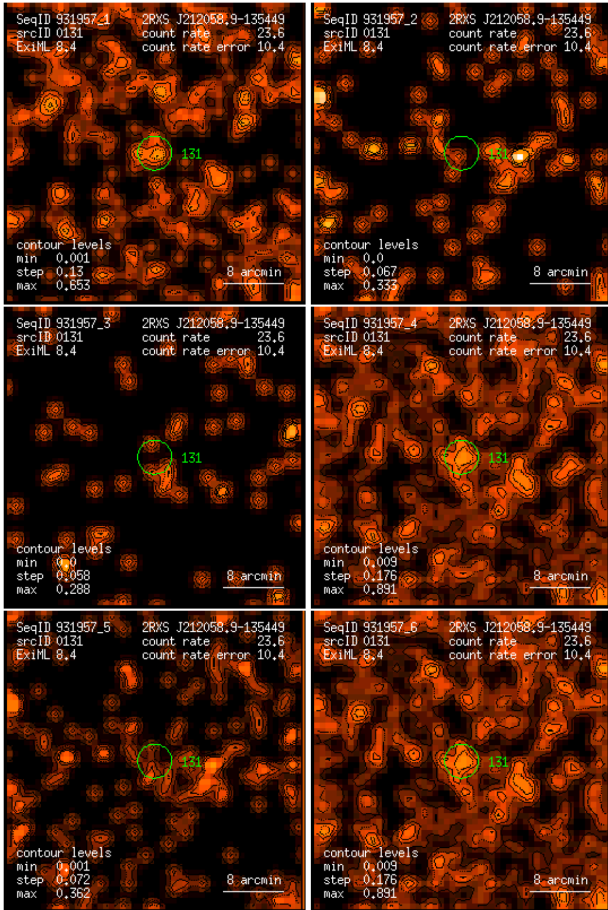
Figure 131: RASS 931957: detection 0131: band rate images, Gaussian filter: (1) PSPC channels 11 – 41, (2) 52 – 90, (3) 91 – 201, (4) 11 – 235, (5) 52 – 201, (6) 11 – 201. Broad band rates in counts/ks. Band rate contour levels in counts/ks/arcmin 2 .
