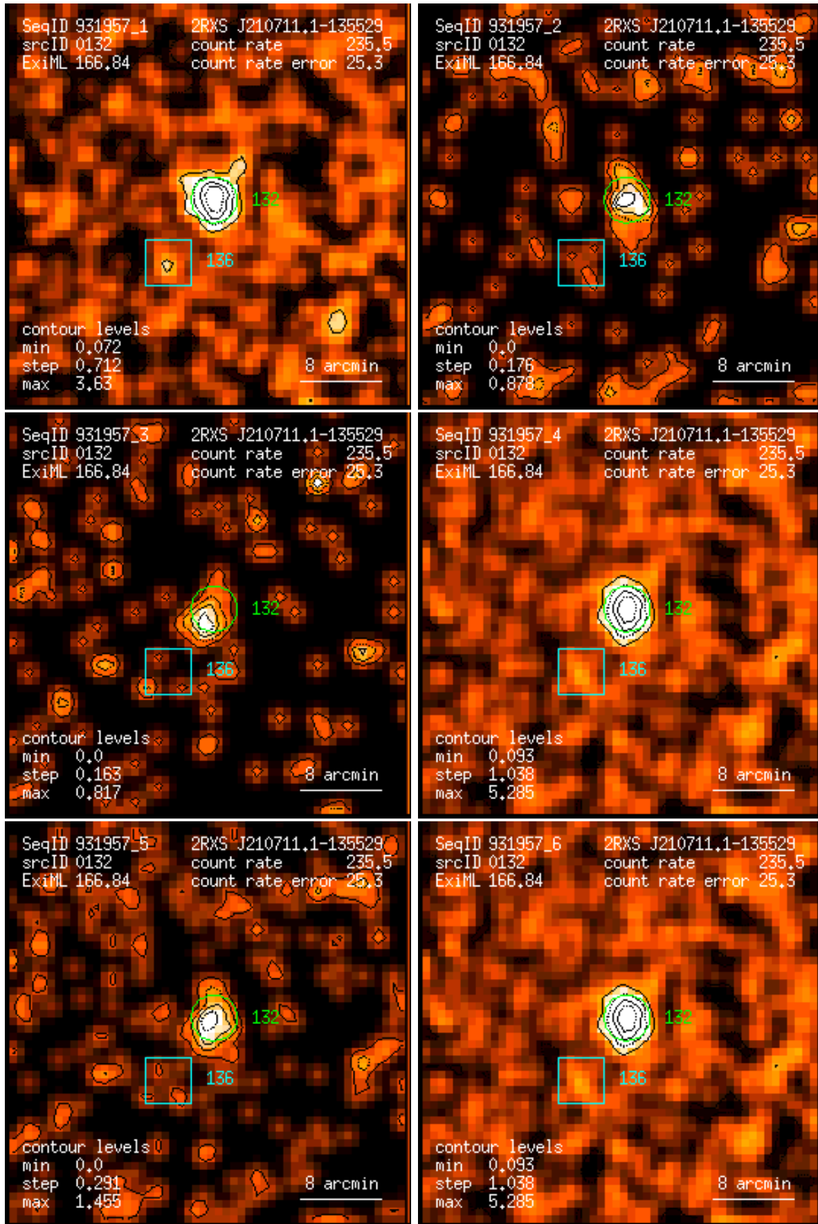
Figure 132: RASS 931957: detection 0132: band rate images, Gaussian filter: (1) PSPC channels 11 – 41, (2) 52 – 90, (3) 91 – 201, (4) 11 – 235, (5) 52 – 201, (6) 11 – 201. Broad band rates in counts/ks. Band rate contour levels in counts/ks/arcmin 2 .
