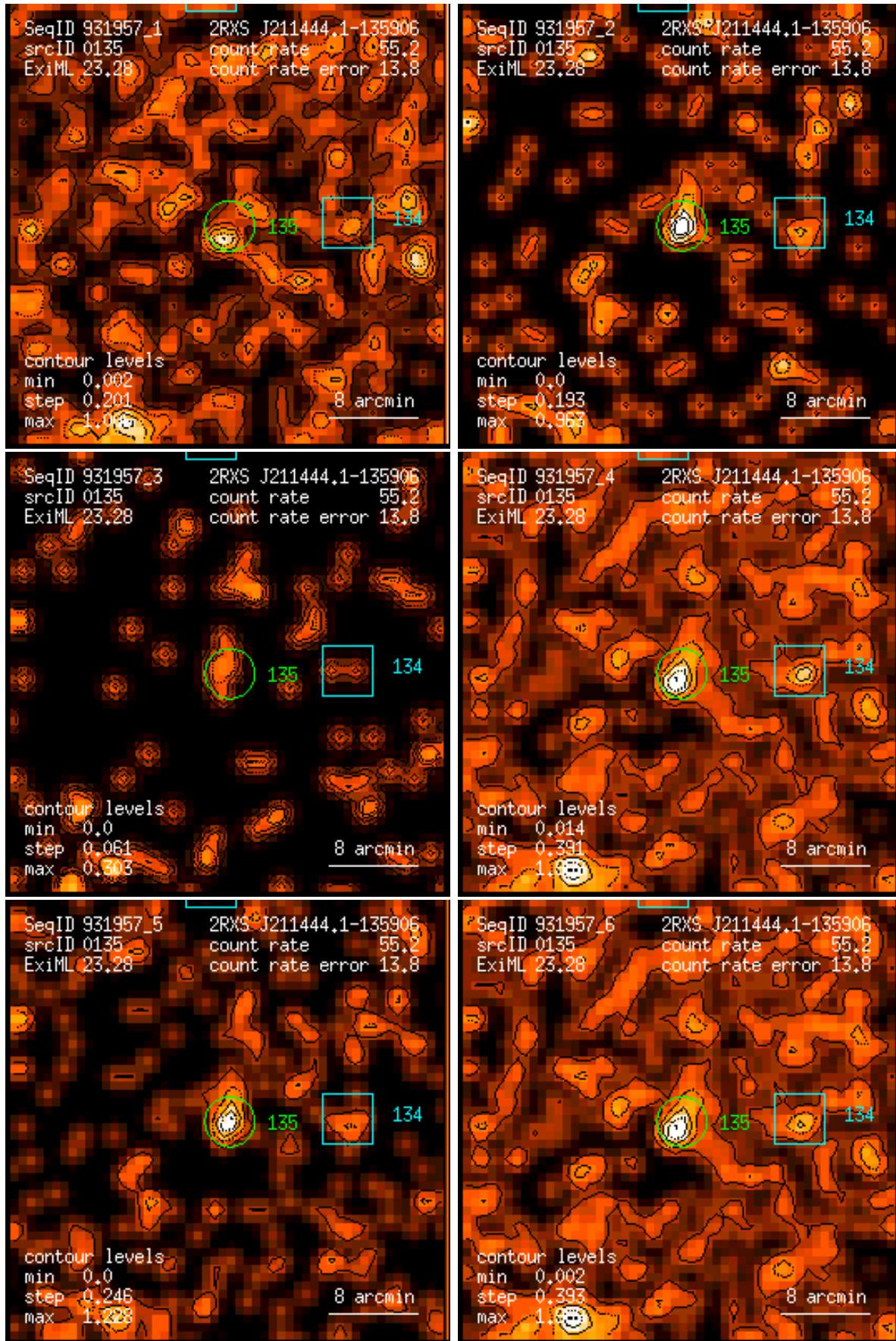
Figure 135: RASS 931957: detection 0135: band rate images, Gaussian filter: (1) PSPC channels 11 – 41, (2) 52 – 90, (3) 91 – 201, (4) 11 – 235, (5) 52 – 201, (6) 11 – 201. Broad band rates in counts/ks. Band rate contour levels in counts/ks/arcmin 2 .
