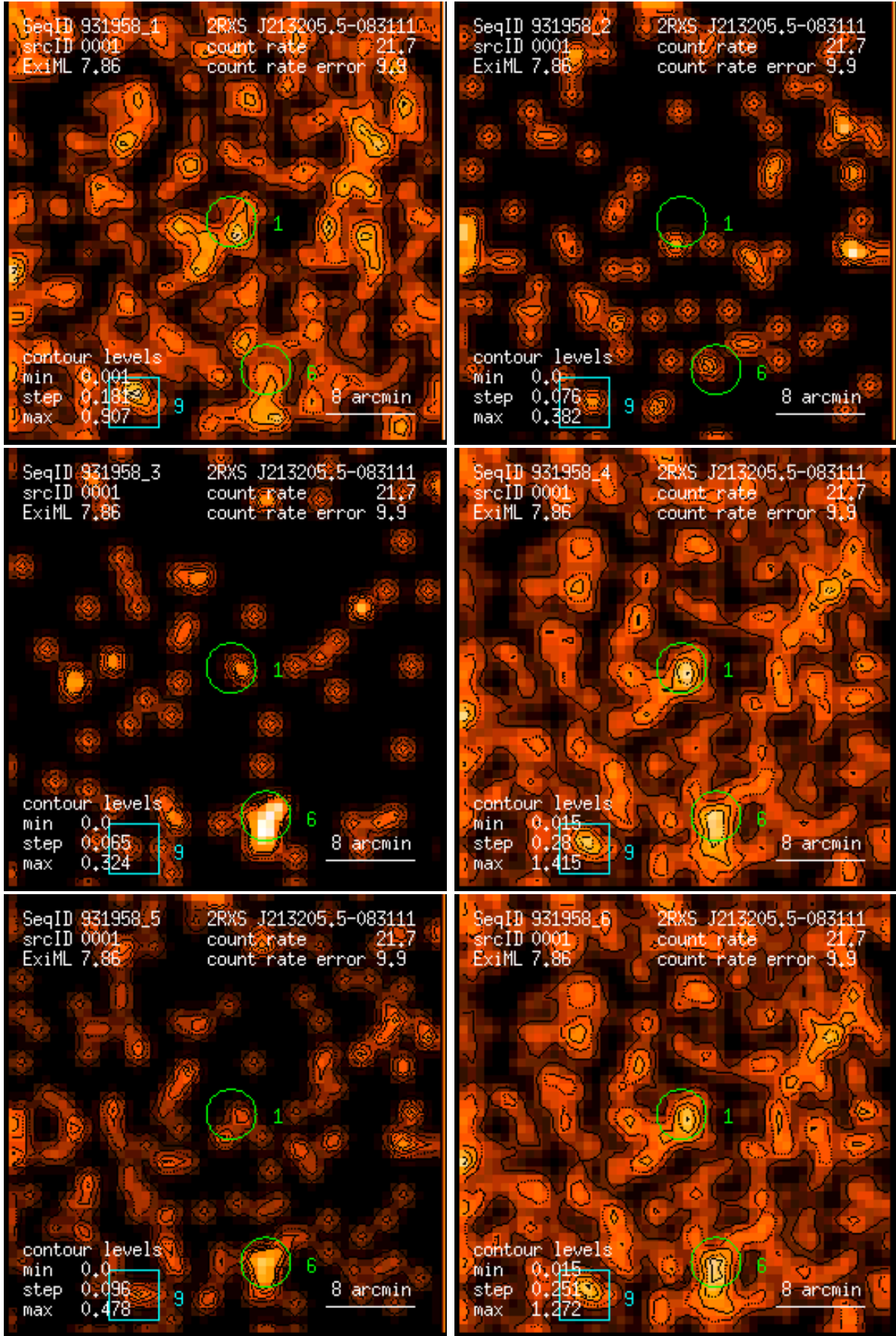
Figure 1: RASS 931958: detection 0001: band rate images, Gaussian filter: (1) PSPC channels 11 – 41, (2) 52 – 90, (3) 91 – 201, (4) 11 – 235, (5) 52 – 201, (6) 11 – 201. Broad band rates in counts/ks. Band rate contour levels in counts/ks/arcmin 2 .
