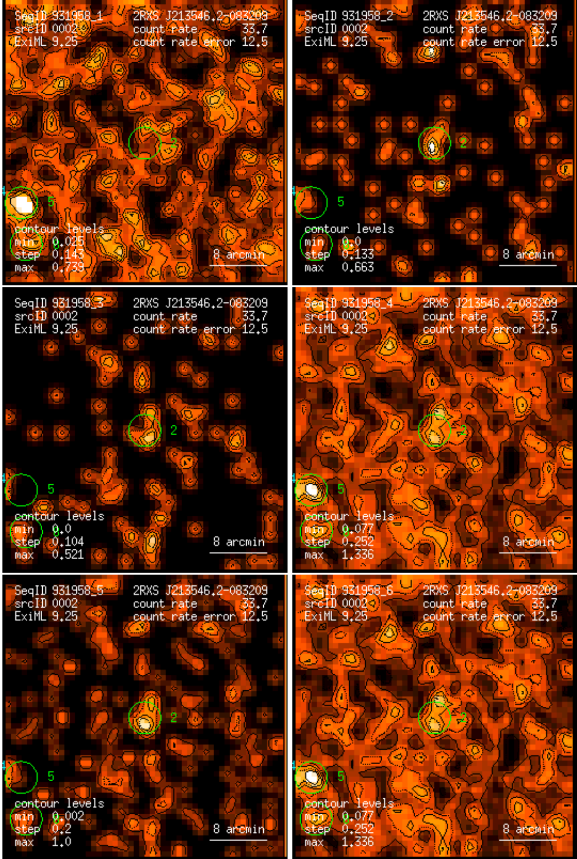
Figure 2: RASS 931958: detection 0002: band rate images, Gaussian filter: (1) PSPC channels 11 – 41, (2) 52 – 90, (3) 91 – 201, (4) 11 – 235, (5) 52 – 201, (6) 11 – 201. Broad band rates in counts/ks. Band rate contour levels in counts/ks/arcmin 2 .
