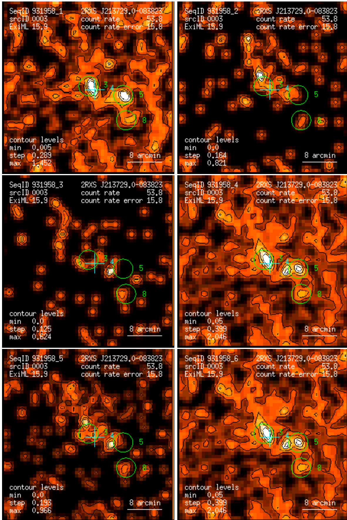
Figure 3: RASS 931958: detection 0003: band rate images, Gaussian filter: (1) PSPC channels 11 – 41, (2) 52 – 90, (3) 91 – 201, (4) 11 – 235, (5) 52 – 201, (6) 11 – 201. Broad band rates in counts/ks. Band rate contour levels in counts/ks/arcmin 2 .
